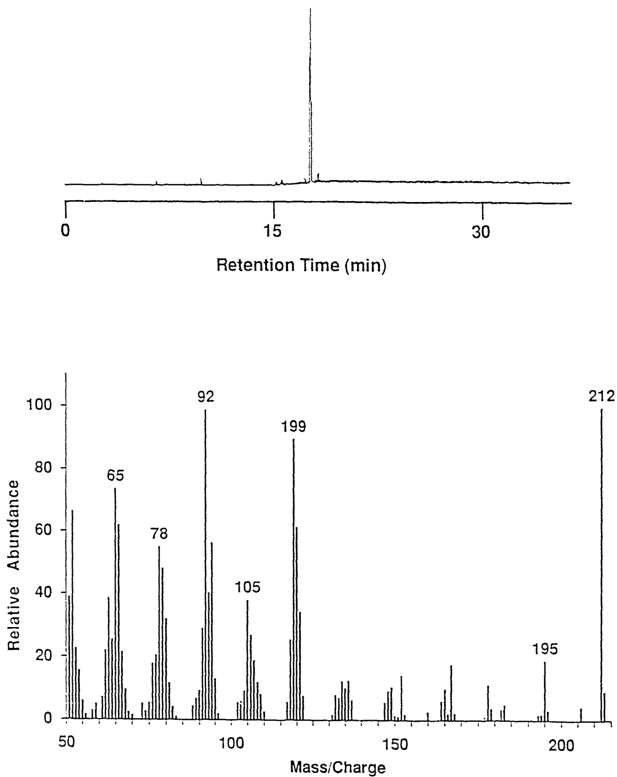
FIGURE 3.14. Total Ion Current Chromatogram (top) of Transformation Product 3 and the Mass Spectrum of the Major Component (bottom)
