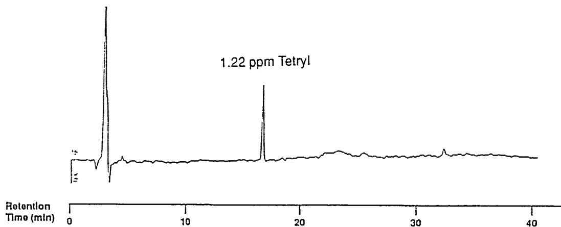
FIGURE 2.7. HPLC Chromatogram of a 1.22-μg/g Tetryl Standard
