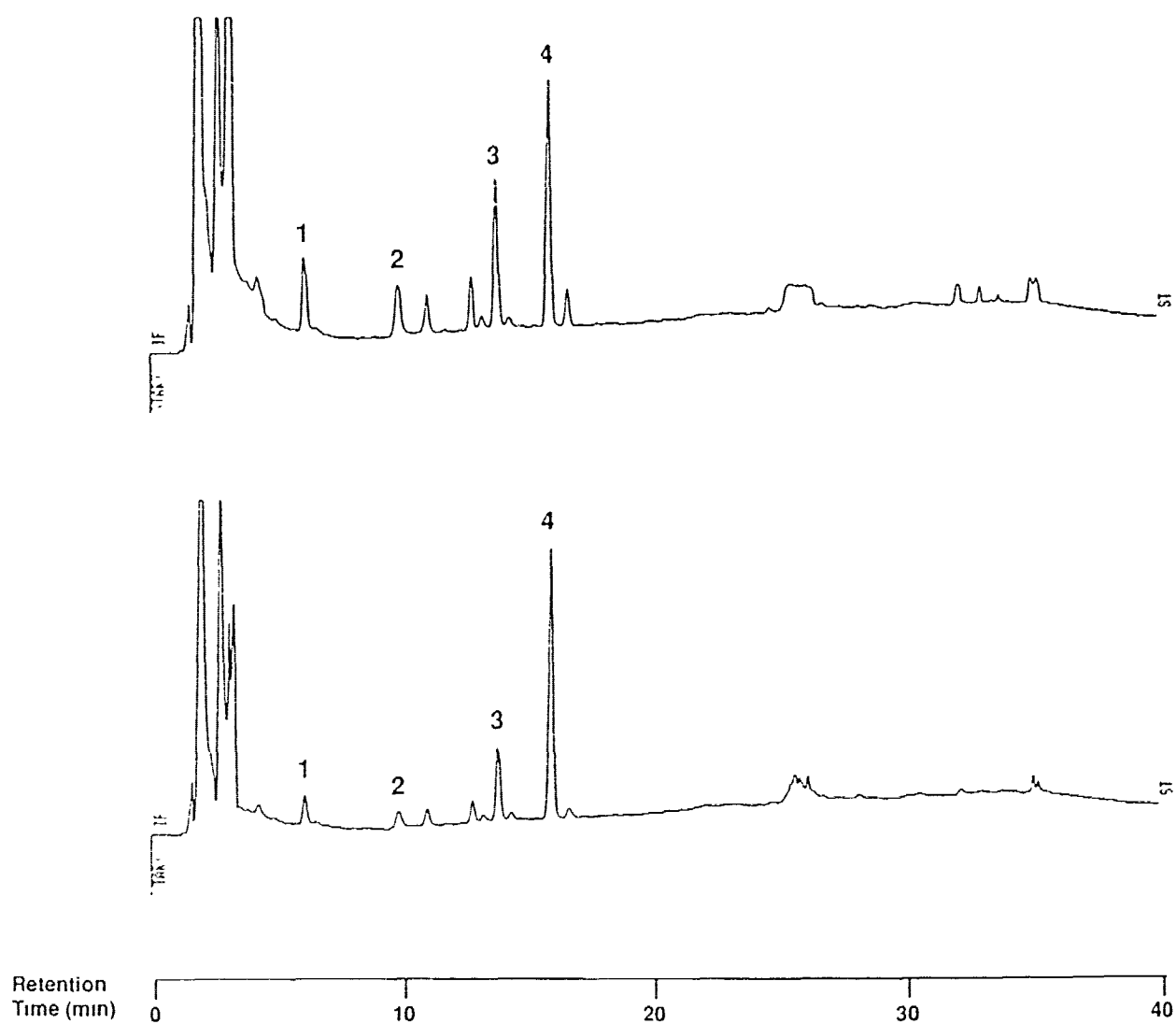
FIGURE 3.13. Chromatographic Profile of an Extract from Palouse Soil Aged 11 Days with Tetraol (top) and a Co-Injection of the Same Extract with Synthetic N -methyl-2,4,6-trinitroaniline (bottom)
