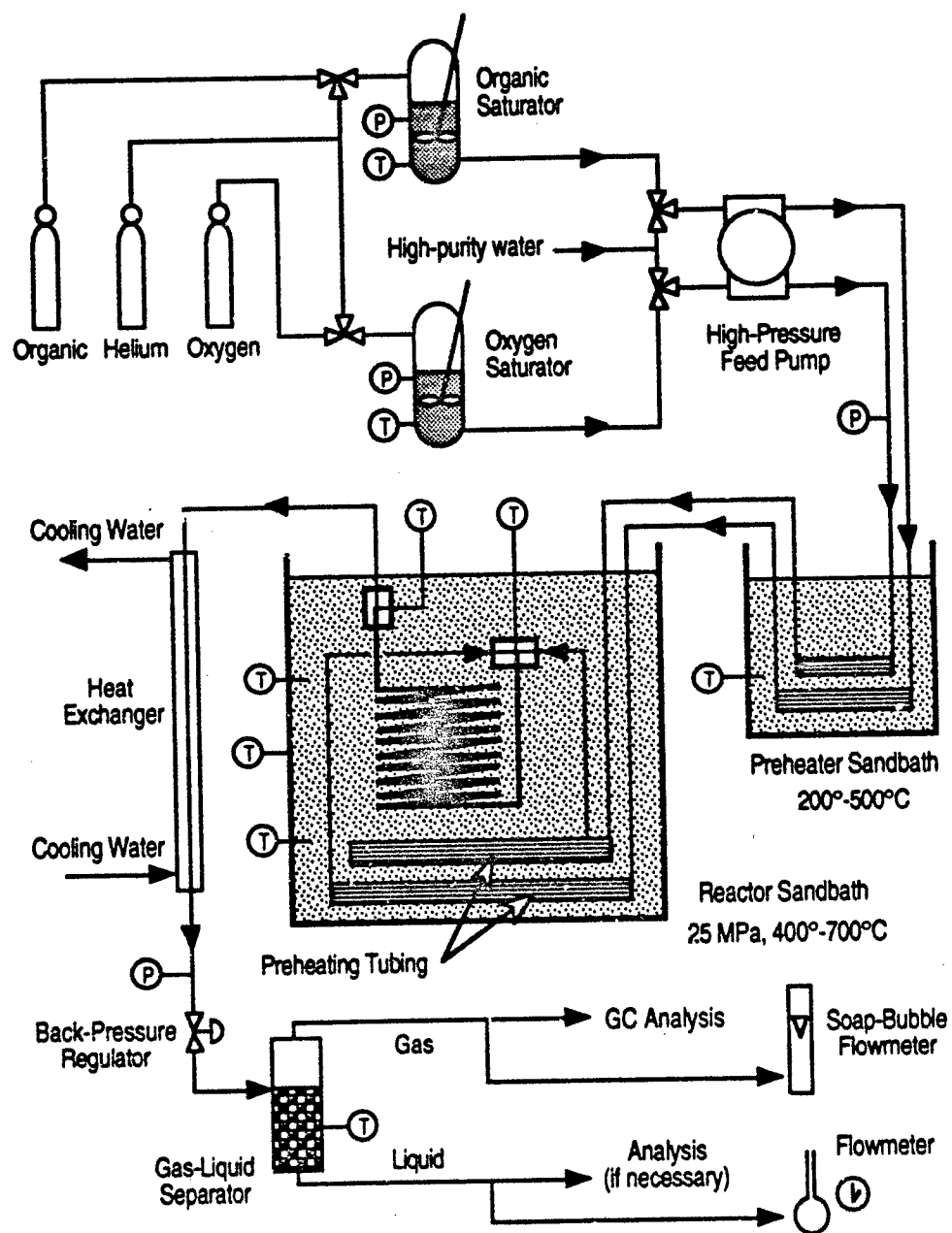
Figure 4.1 Isothermal, Plug-Flow Reactor Apparatus. From Holgate (1993).
