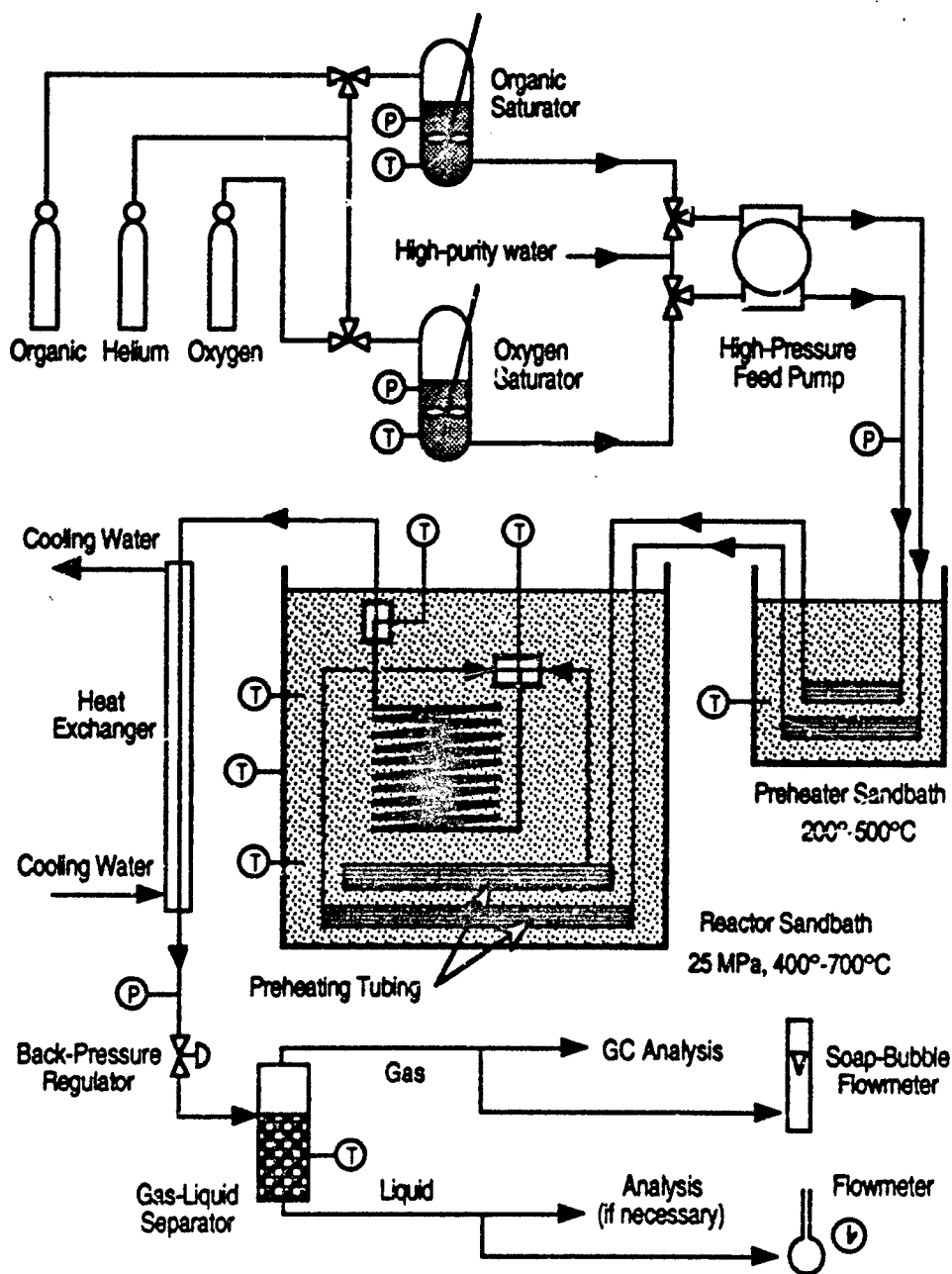
Figure 1.1 Isothermal, Plug-Flow Reactor Apparatus.
