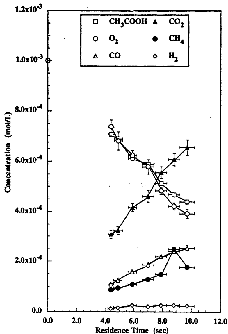
Figure 6.14 Major Species Profiles for Oxygen-Lean Acetic Acid Oxidation in Supercritical Water at 525 °C and 246 bar. [O_2]_0 = (1.09 \pm 0.2) \times 10^{-3} mol/L, [CH_3COOH]_0 = (0.98 \pm 0.01) \times 10^{-3} mol/L. Error bars represent 95% confidence intervals.
