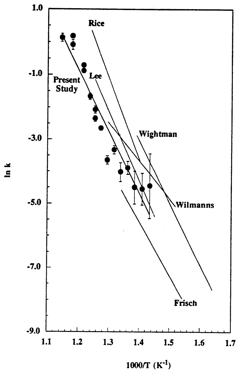
Figure 6.1 Comparison of First-Order Arrhenius Plots for Oxidation of Acetic Acid in Supercritical Water. Data points shown are from this present study. Error bars represent 95% confidence intervals.
