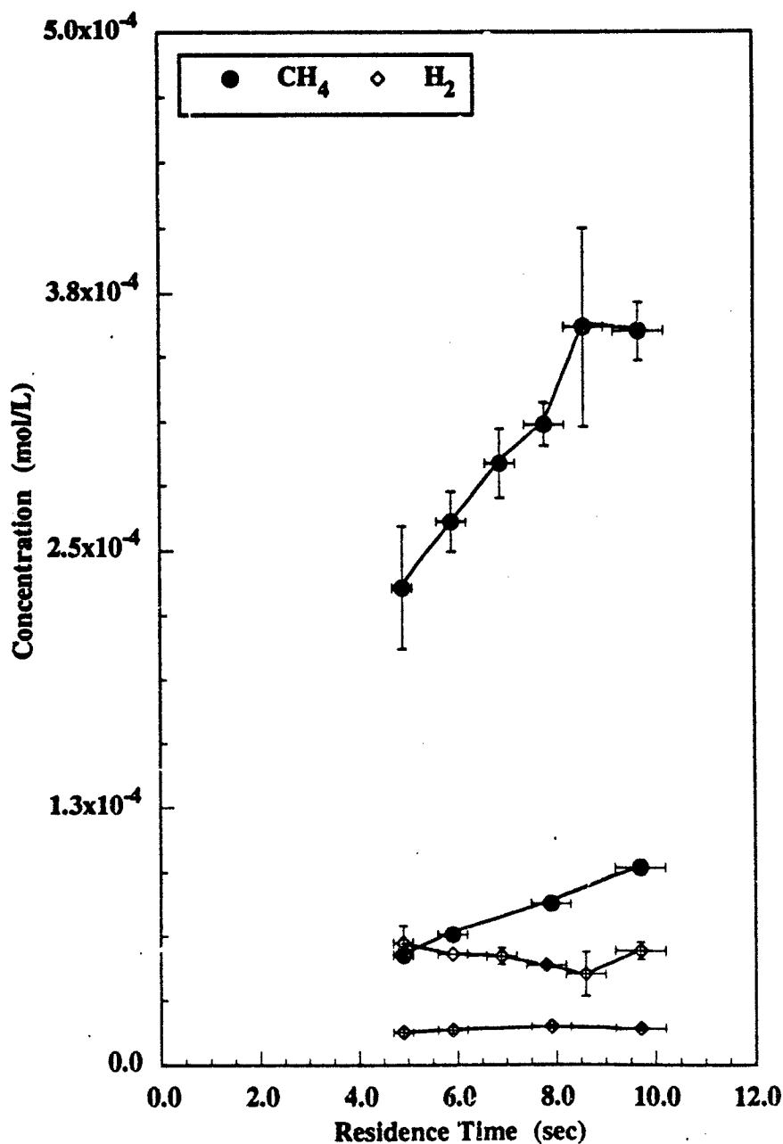
Figure 6.13 Comparison of Methane and Hydrogen Profiles for Stoichiometric (1:0.5 and 4:2) Acetic Acid Oxidation in Supercritical Water at 525 °C and 246 bar. Actual average [O_2]_0:[CH_3COOH]_0 feed concentrations are ([1.09 \pm 0.2]:[0.50 \pm 0.01]) \times 10^{-3} mol/L for the lower profile of each species and ([3.90 \pm 0.5]:[2.02 \pm 0.02]) \times 10^{-3} mol/L for the higher profile of each species. Error bars represent 95% confidence intervals.
