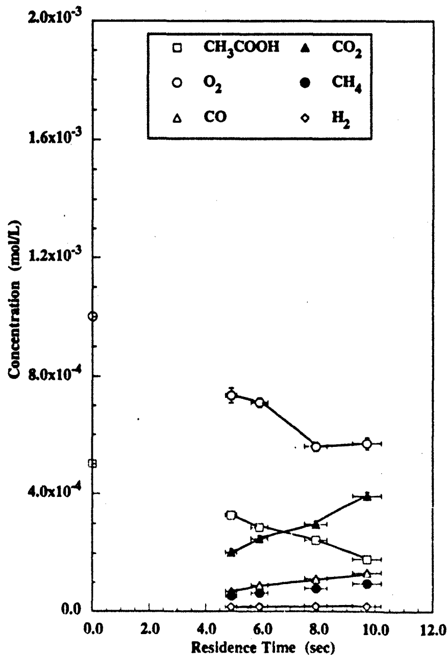
Figure 6.8 Major Species Profiles for Stoichiometric Acetic Acid Oxidation in Supercritical Water at 525 °C and 246 bar. [O_2]_0 = (1.09 \pm 0.2) \times 10^{-3} mol/L, [CH_3COOH]_0 = (0.50 \pm 0.01) \times 10^{-3} mol/L. Error bars represent 95% confidence intervals.
