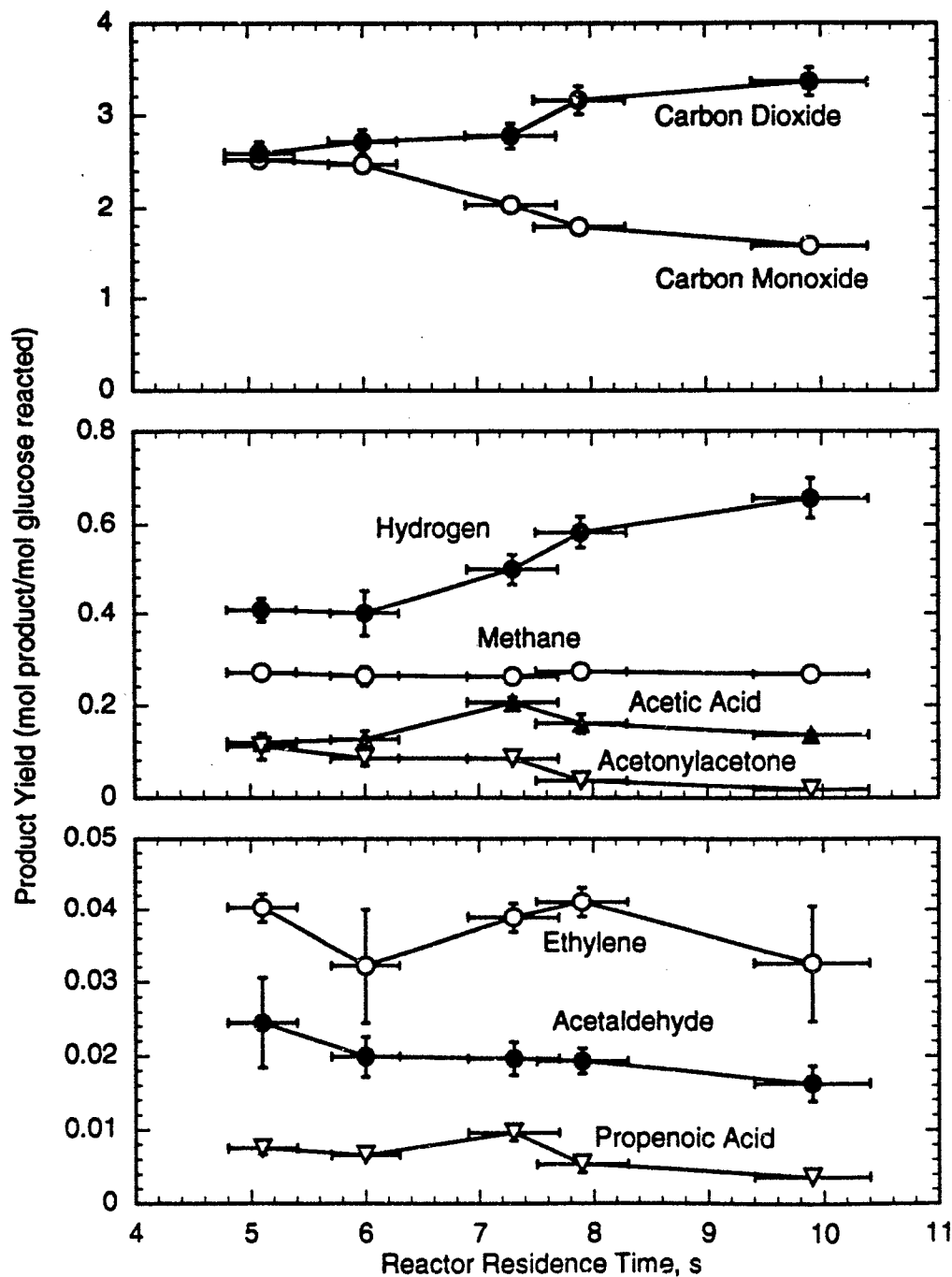
Figure 5.6 Variation of Product Yields with Residence Time for Glucose Oxidation at 500 \pm 2 °C at 246 bar. Experimental conditions: (1.01 \pm 0.02) \times 10^{-3} mol/L glucose, (6.1 \pm 0.2) \times 10^{-3} mol/L oxygen. Error bars represent a 95% confidence interval. From Holgate (1993).
