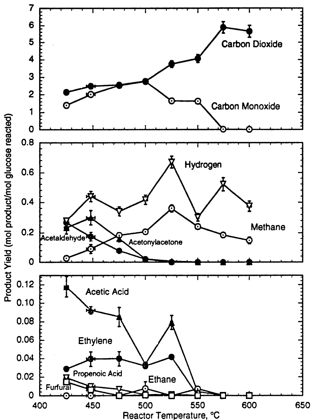
Figure 5.5 Variation of Product Yields with Temperature for Glucose Oxidation at 246 bar. Experimental conditions: (0.99 \pm 0.02) \times 10^{-3} mol/L glucose, (6.2 \pm 0.2) \times 10^{-3} mol/L oxygen, 5.9 \pm 0.3 seconds reactor residence time. Error bars represent a 95% confidence interval. From Holgate (1993).
