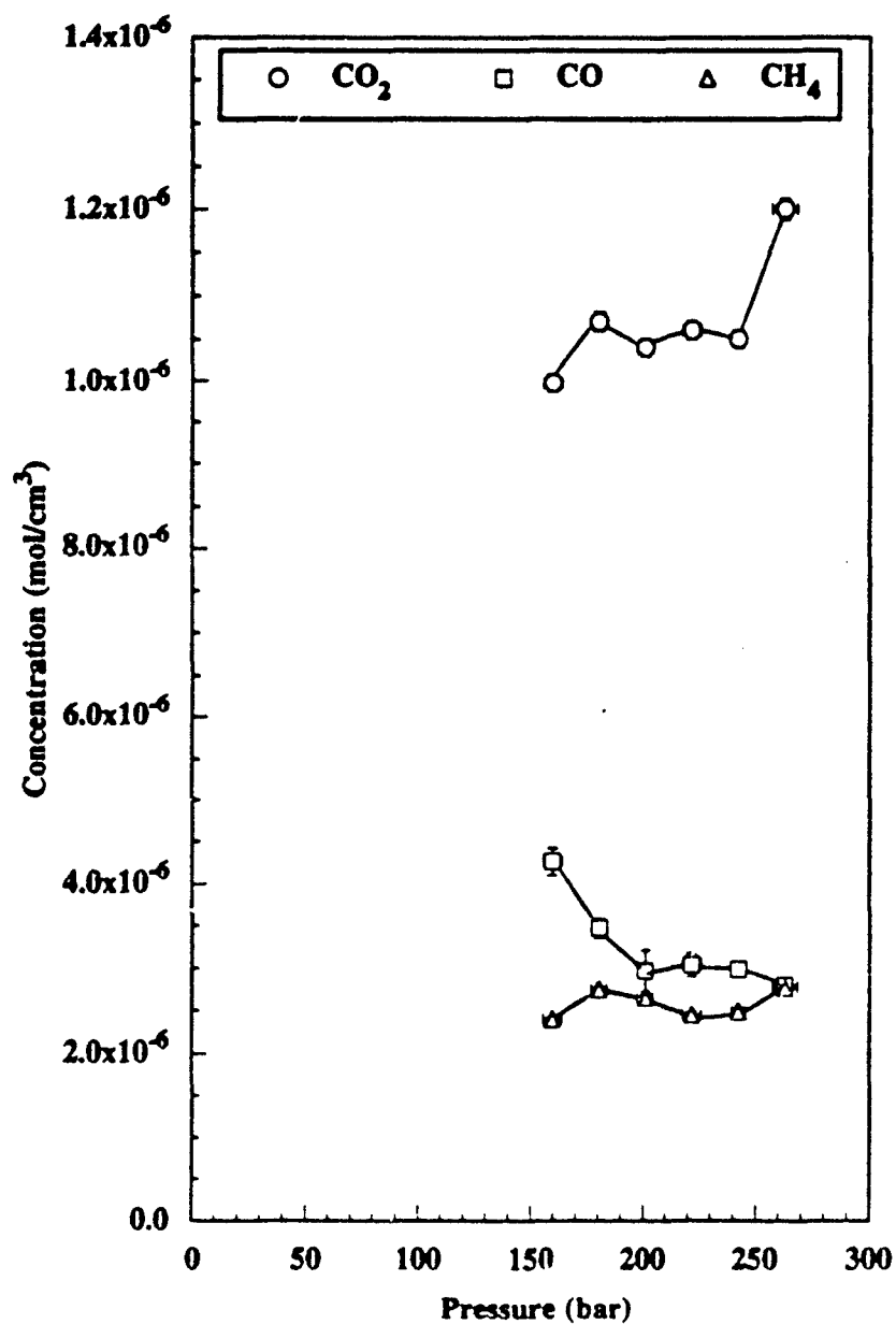
Figure 6.20 Variation with Operating Pressure (Fluid Density) of Major Gaseous Species Concentrations at 550 °C and 4 seconds Residence Time. [\text{CH}_3\text{COOH}]_0 = (0.95 \pm 0.01) \times 10^{-6} \text{ mol/cm}^3 ; [\text{O}_2]_0 = (2.09 \pm 0.02) \times 10^{-6} \text{ mol/cm}^3 .
