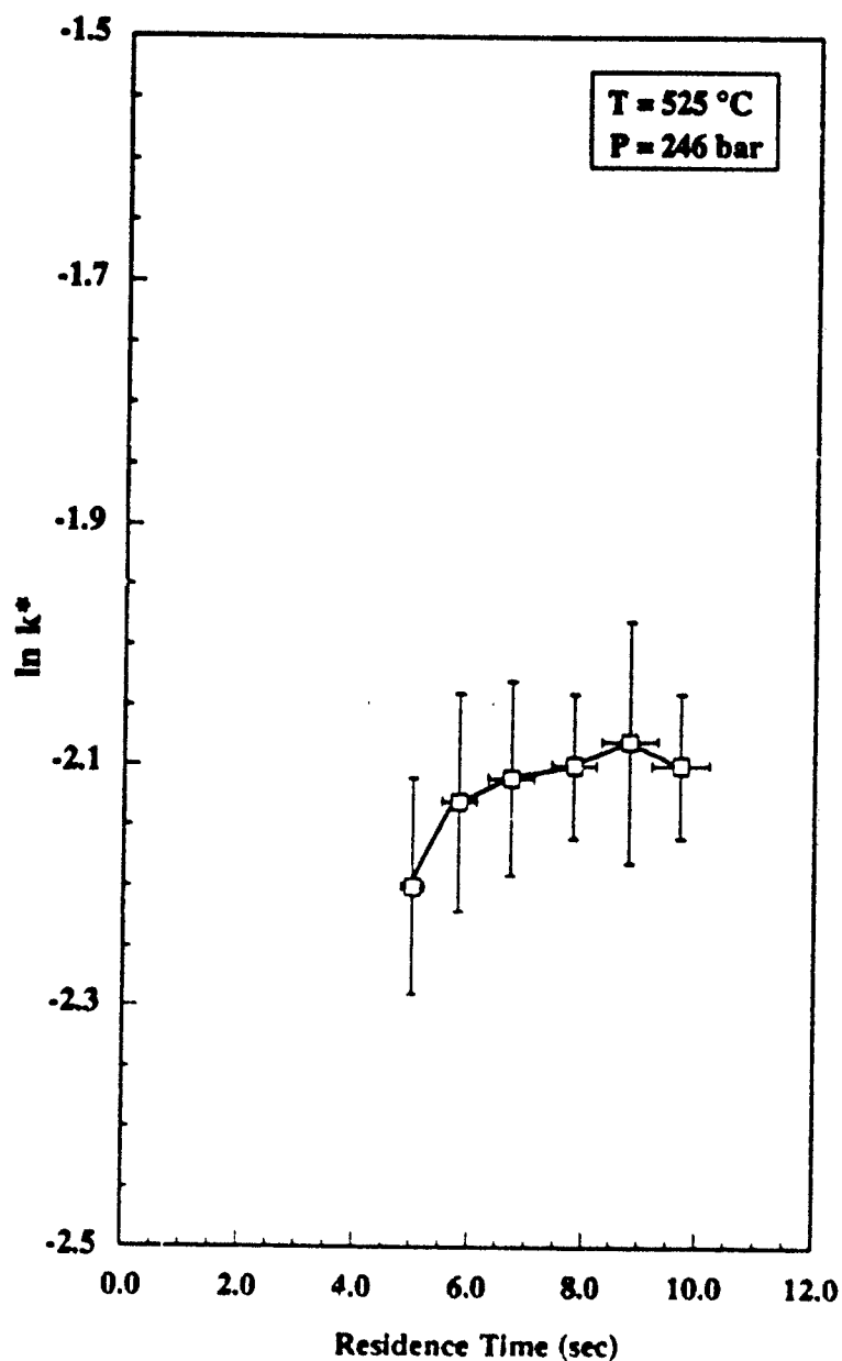
Figure 6.19 Variation of the Apparent First-Order Rate Constant, k^* , with Residence Time. Experimental Conditions: [\text{CH}_3\text{COOH}]_0 = (2.02 \pm .02) \times 10^{-6} \text{ mol/cm}^3 ; [\text{O}_2]_0 = (3.90 \pm .05) \times 10^{-6} \text{ mol/cm}^3 . 95% confidence intervals are shown.
