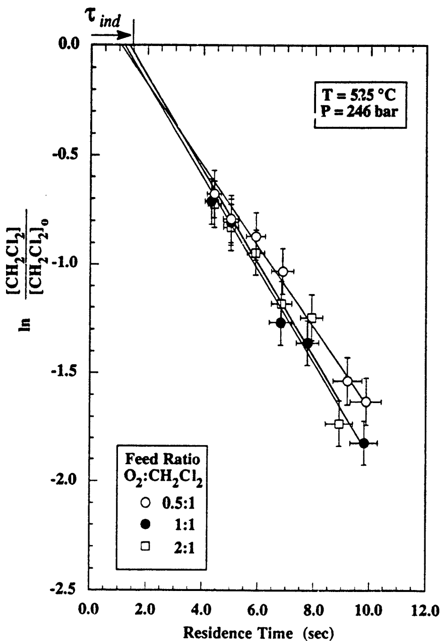
Figure 1.4 Normalized Decay Profiles for Stoichiometric Oxidation of Methylene Chloride in Supercritical Water at 525 °C and 246 bar, Showing Induction Times. Conditions as in Figure 7.6, but concentration ordinate is on alogarithmic scale. Lines are linear fits to data, indicating exponential decay.
