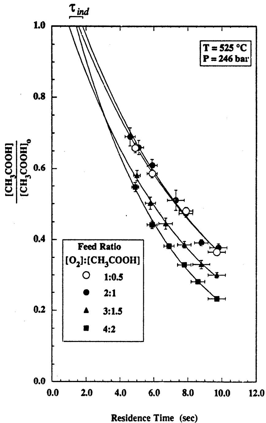
Figure 6.3 Normalized Decay Profiles for Stoichiometric Oxidation of Acetic Acid in Supercritical Water, Showing Induction Times. Curves are exponential fits to data points.
