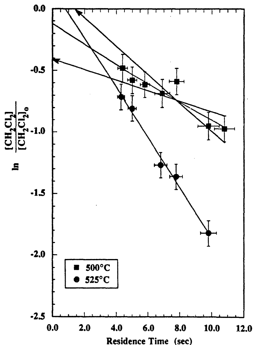
Figure 7.8 Normalized Decay Profiles for Oxidation of Methylene Chloride in Supercritical Water at 525 °C and 500 °C with Pressure of 246 bar. Concentration ordinate is on a logarithmic scale. Nominal feed concentrations are 1 \times 10^{-6} mol/cm 3 for both O 2 and CH 2 Cl 2 . Lines are linear fits to data, suggesting exponential decay. Error bars represent 95% confidence intervals. Arrows indicate approximate 95% limit of confidence on the slope of the line through data at 500 °C.
