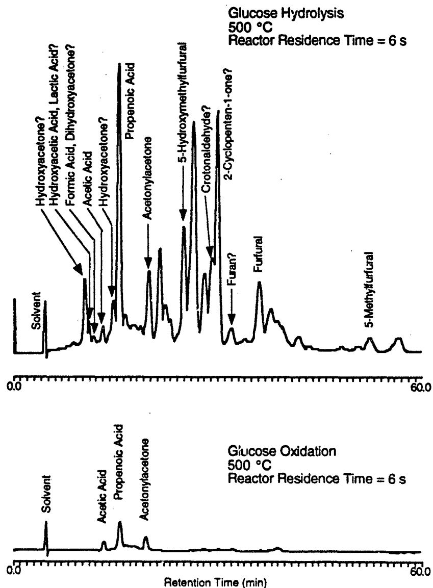
Figure 5.1 Comparison of HPLC Chromatograms of Liquid Effluent from Glucose Hydrolysis and Oxidation in Supercritical Water. Nominal initial conditions: 500 °C, 1 \times 10^{-6} mol/cm 3 glucose, 6 \times 10^{-6} mol/cm 3 oxygen (for oxidation), 6 seconds reactor residence time. UV detection at 210 nm. From Holate (1993).
