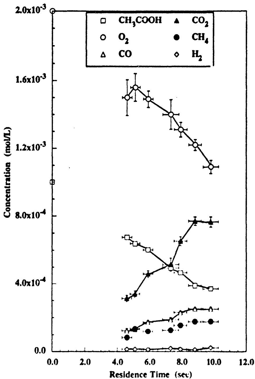
Figure 6.7 Major Species Profiles for Stoichiometric Acetic Acid Oxidation in Supercritical Water at 525 °C and 246 bar. [O_2]_0 = (2.08 \pm 0.4) \times 10^{-3} mol/L, [CH_3COOH]_0 = (0.98 \pm 0.01) \times 10^{-3} mol/L. Error bars represent 95 % confidence intervals.
