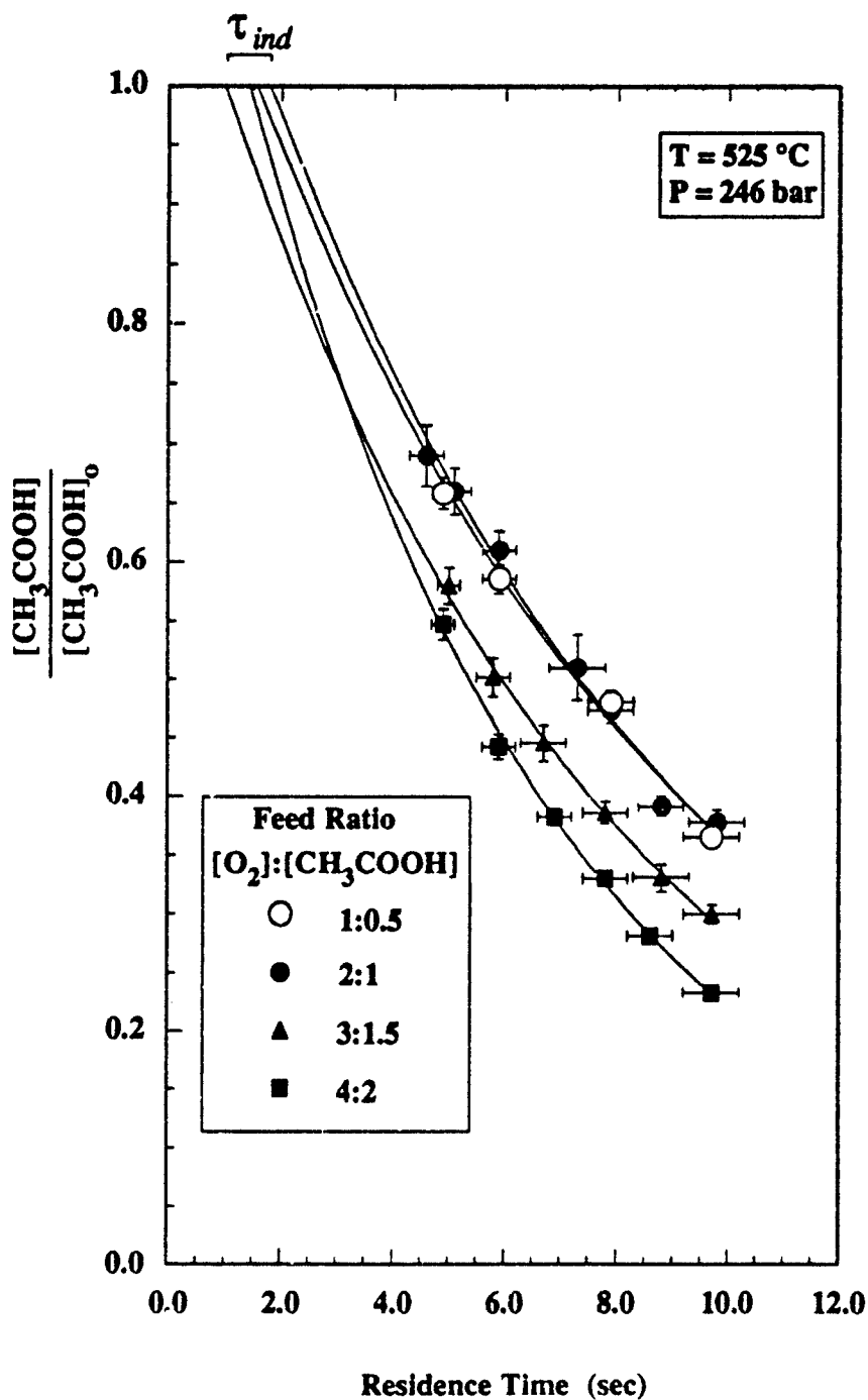
Figure 1.2 Normalized Decay Profiles for Stoichiometric Oxidation of Acetic Acid in Supercritical Water, Showing Induction Times. Curves are exponential fits to data points.
