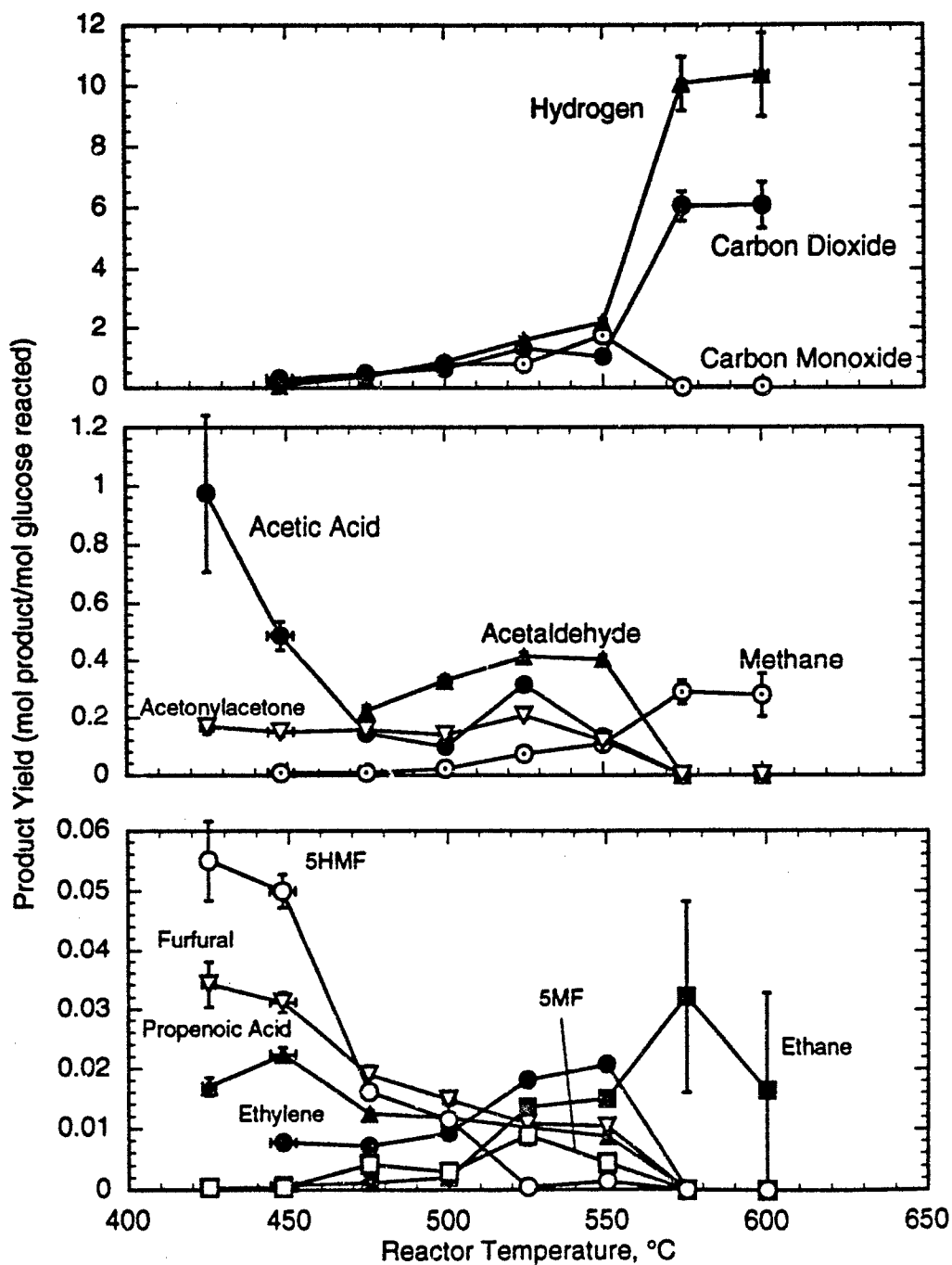
Figure 5.4 Variation of Product Yields with Temperature for Glucose Hydrolysis at 246 bar. Experimental conditions: (1.02 \pm 0.02) \times 10^{-3} mol/L glucose, 6.1 \pm 0.3 seconds reactor residence time. Error bars represent a 95% confidence interval. From Holgate (1993).
