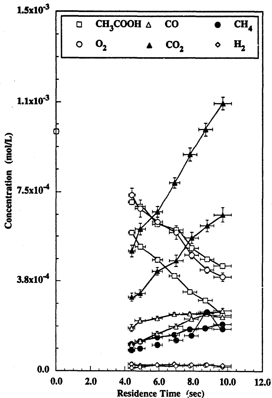
Figure 6.16 Combined Major Species Profiles for Oxygen-Lean and Oxygen-Rich Acetic Acid Oxidation in Supercritical Water at 525 °C and 246 bar. (Figures 6.14 and 6.15 combined) Error bars represent 95% confidence intervals.
