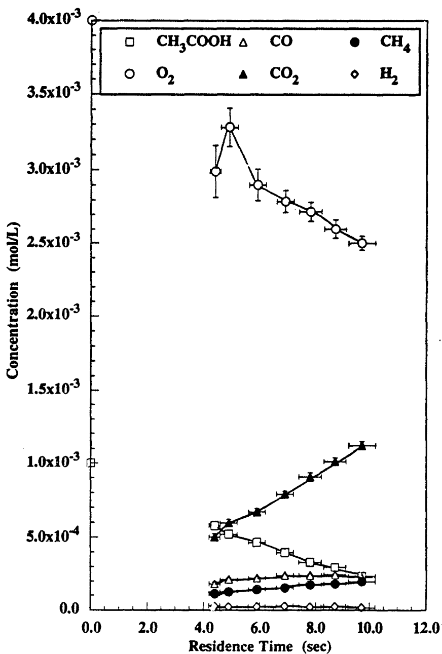
Figure 6.15 Major Species Profiles for Oxygen-Rich Acetic Acid Oxidation in Supercritical Water at 525 °C and 246 bar. [O_2]_0 = (3.86 \pm 0.4) \times 10^{-3} mol/L, [CH_3COOH]_0 = (0.99 \pm 0.01) \times 10^{-3} mol/L. Error bars represent 95% confidence intervals.
