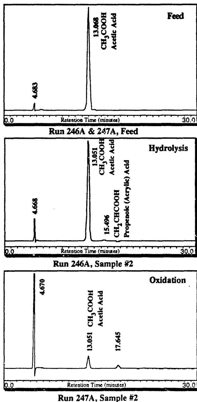
Figure 6.24 Comparison of Liquid Effluent Chromatograms in Acetic Acid Hydrolysis and Oxidation Experiments. Experimental conditions: 550°C, 246 bar, 8 seconds residence time, with [\text{CH}_3\text{COOH}]_0 = (1.00 \pm 0.03) \times 10^{-6} \text{ mol/cm}^3 and [\text{O}_2]_0 = (2.03 \pm 0.07) \times 10^{-6} \text{ mol/cm}^3 for oxidation.
