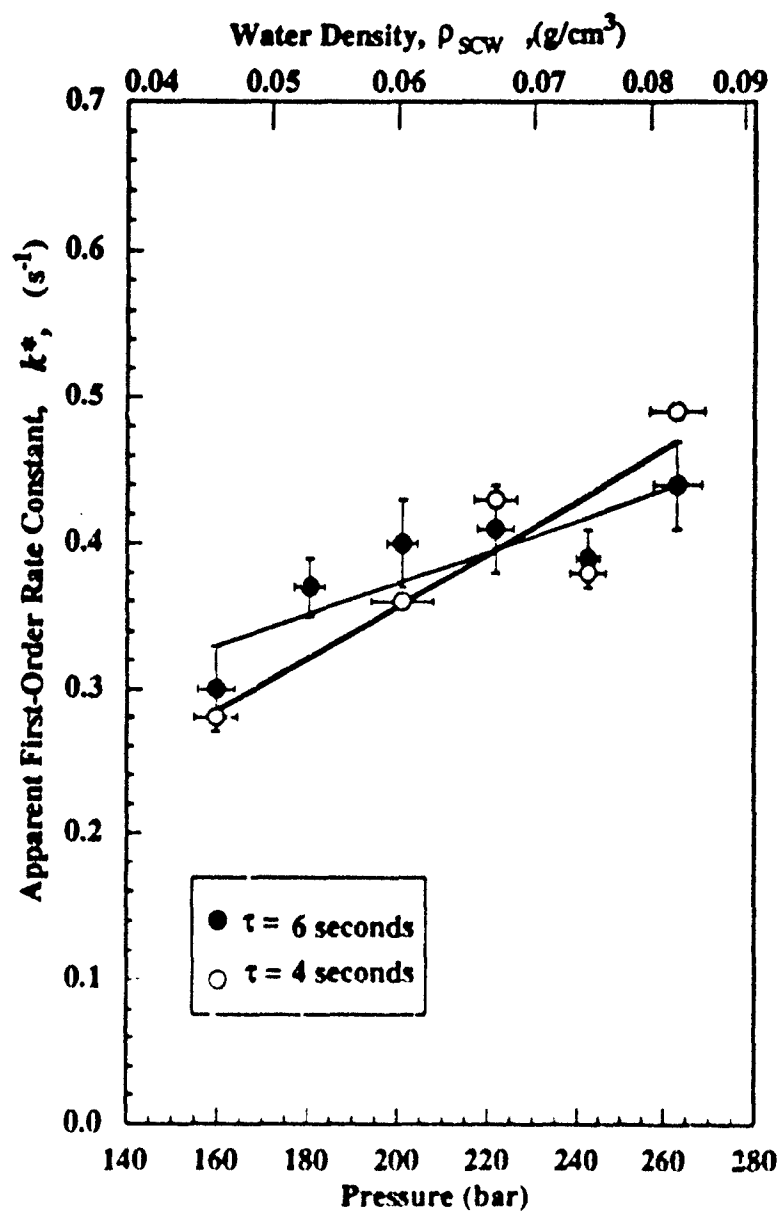
Figure 6.18 Effects of Operating Pressure (Fluid Density) on the Apparent First-Order Rate Constant, k^* , for Acetic Acid Oxidation at 550 °C. Experimental Conditions: [\text{CH}_3\text{COOH}]_0 = (0.95 \pm 0.01) \times 10^{-6} \text{ mol/cm}^3 ; [\text{O}_2]_0 = (2.09 \pm 0.02) \times 10^{-6} \text{ mol/cm}^3 . 95% confidence intervals are shown.
