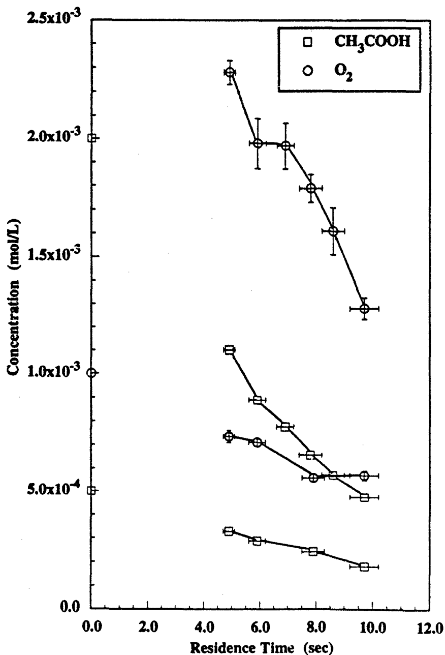
Figure 6.11 Comparison of Acetic Acid and Oxygen Profiles for Stoichiometric (1:0.5 and 4:2) Acetic Acid Oxidation in Supercritical Water at 525 °C and 246 bar. Actual average [O_2]_0:[CH_3COOH]_0 feed concentrations are ([1.09 \pm 0.2]:[0.50 \pm 0.01]) \times 10^{-3} mol/L for the lower profile of each species and ([3.90 \pm 0.5]:[2.02 \pm 0.02]) \times 10^{-3} mol/L for the higher profile of each species. Error bars represent 95% confidence intervals.
