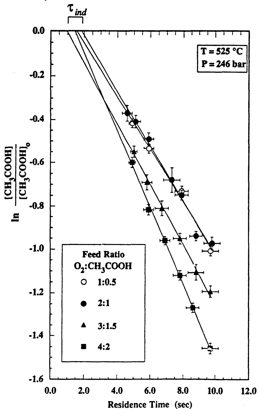
Figure 6.4 Normalized Decay Profiles for Stoichiometric Oxidation of Acetic Acid in Supercritical Water at 525 °C and 246 bar, Showing Induction Times. Conditions as in Figure 6.3, but concentration ordinate is on a logarithmic scale. Lines are linear fits to data, indicating exponential decay.
