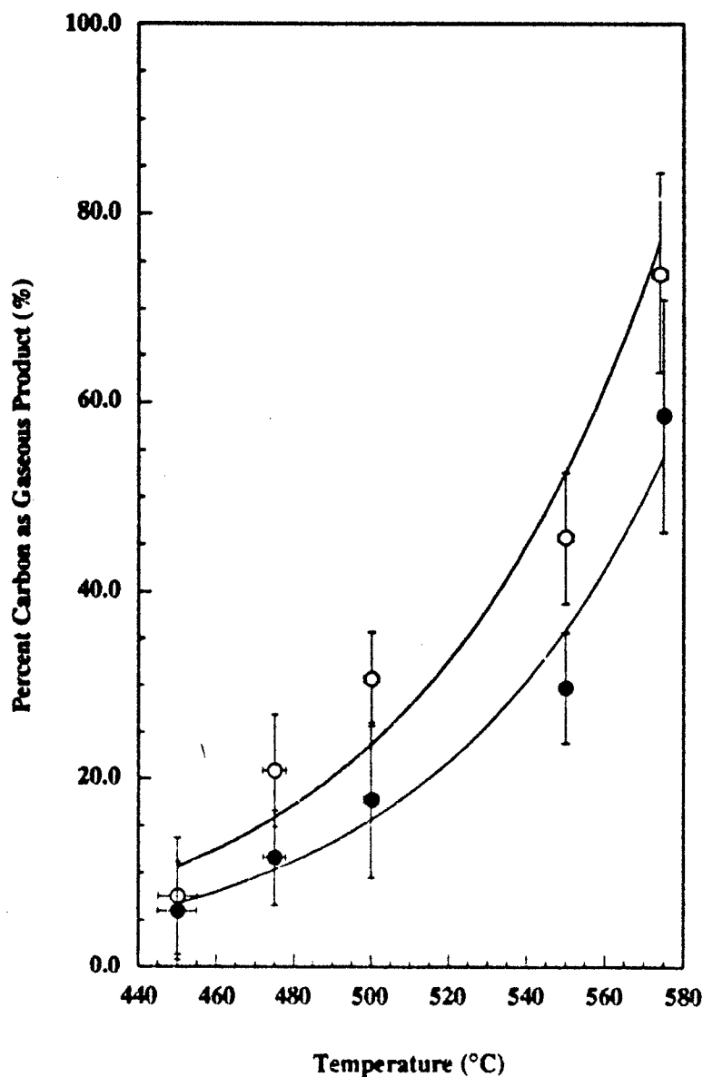
Figure 7.4 Percent of Reacted Carbon that Appears as Gas Phase Product in Methylene Chloride Hydrolysis and Oxidation in Supercritical Water. Reactor pressure of 246 bar and residence time of 6 seconds. [\text{CH}_2\text{Cl}_2]_0 = 1 \times 10^{-6} \text{ mol/cm}^3 for hydrolysis and oxidation; [\text{O}_2]_0 = 1 \times 10^{-6} \text{ mol/cm}^3 for oxidation. Exponential fits for clarity only.
