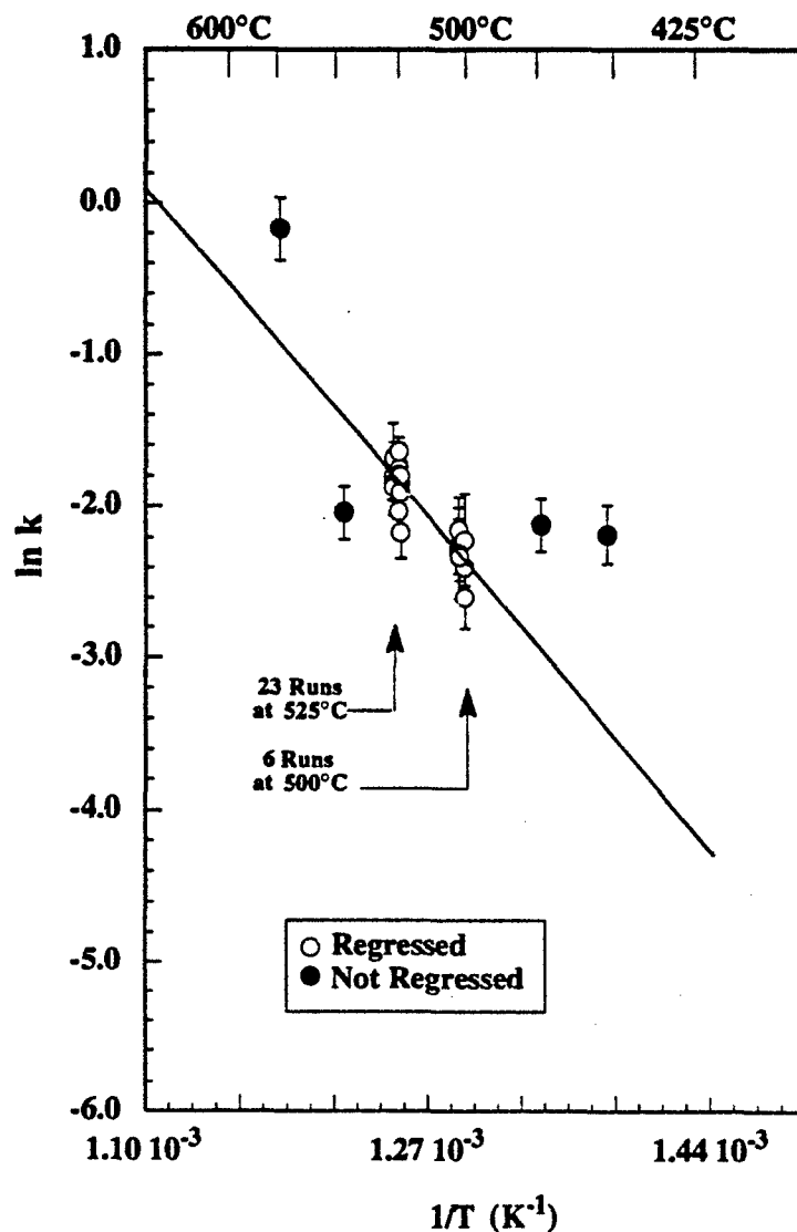
Figure 7.5 Assumed First-Order Arrhenius Plot for Methylene Chloride Oxidation in Supercritical Water at 246 bar. Linear least squares fit is shown, corresponding to Equation 7.7. Data represent the combined effect of hydrolysis and oxidation, which occur simultaneously. Error bars represent 95% confidence intervals.
