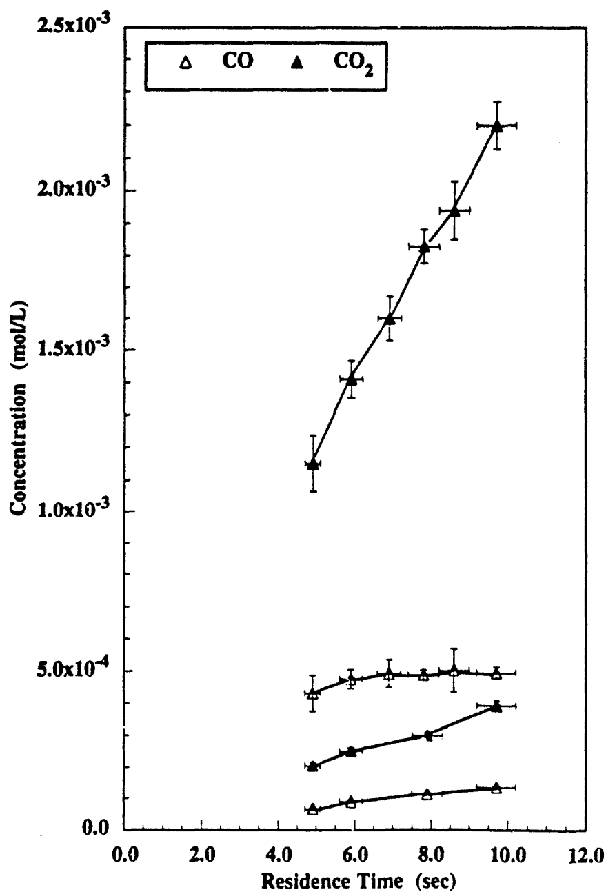
Figure 6.12 Comparison of Carbon Monoxide and Carbon Dioxide Profiles for Stoichiometric (1:0.5 and 4:2) Acetic Acid Oxidation in Supercritical Water at 525 °C and 246 bar. Actual average [O_2]_0:[CH_3COOH]_0 feed concentrations are ([1.09 \pm 0.2]:[0.50 \pm .01]) \times 10^{-3} mol/L for the lower profile of each species and ([3.90 \pm 0.5]:[2.02 \pm .02]) \times 10^{-3} mol/L for the higher profile of each species.
