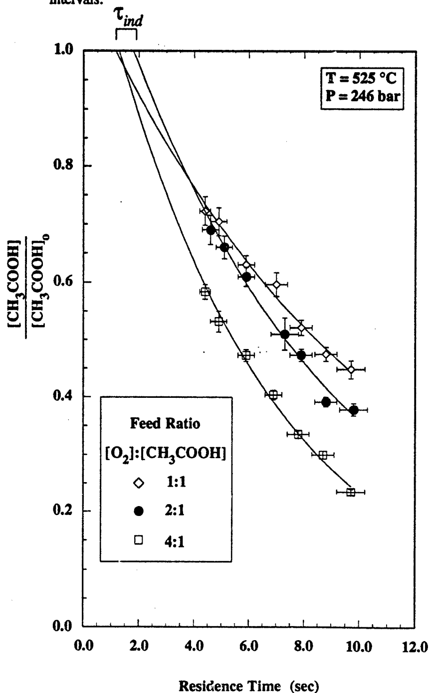
Figure 6.5 Normalized Decay Profiles for Oxidation of Acetic Acid in Supercritical Water at 525 °C and 246 bar, Showing Induction Times. Curves are exponential fits. Error bars represent 95% confidence intervals.
