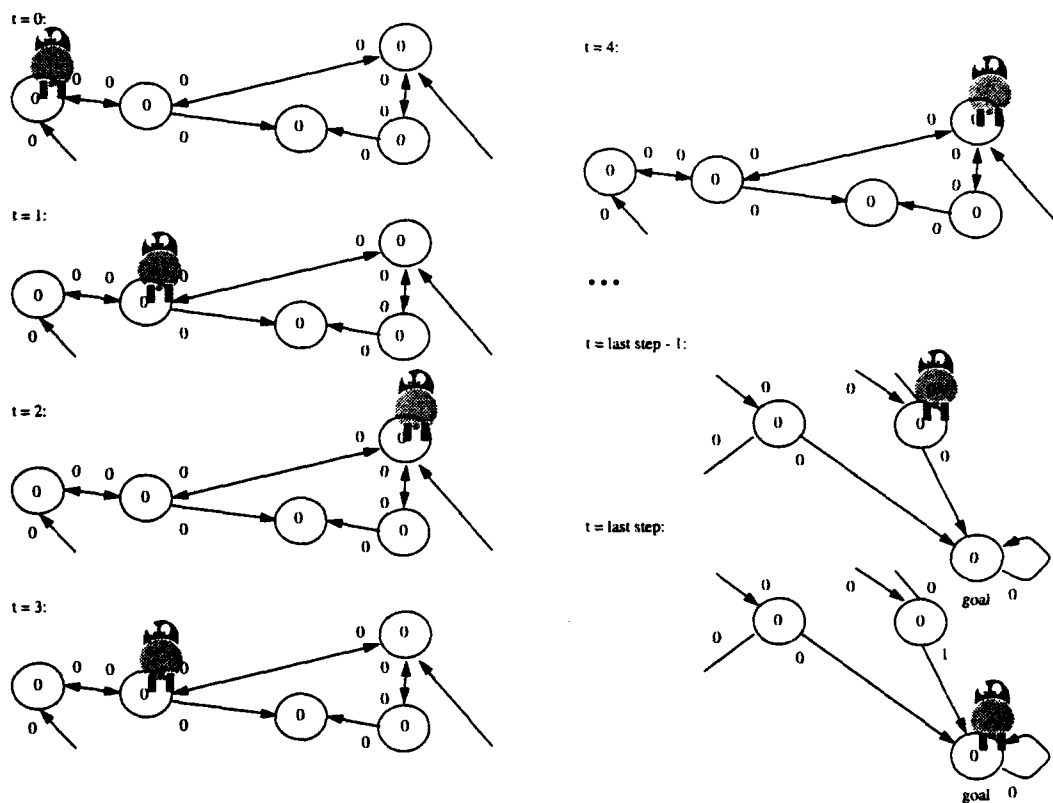
Figure 7: Possible trace of the agent if goal-reward representation is used
