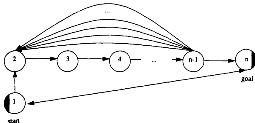
Figure 14: A domain for which an admissible, zero-initialized Q-learning algorithm (and every other uninformed on-line search algorithm) can need at least (e - n)(n - 2) + 1 steps to reach the goal state, but an off-line search algorithm that knows the topology of the state space needs only one step to reach the goal state (for n \geq 3 and e \geq n + 1 )
