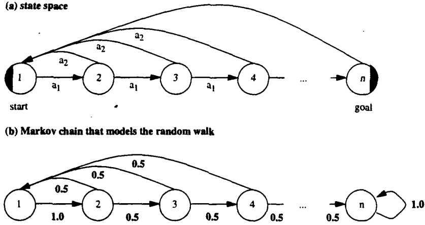
Figure 8: A domain (“reset state space”) for which a random walk needs 3 \times 2^{n-2} - 2 steps on average to reach the goal state (for n \geq 2 )
