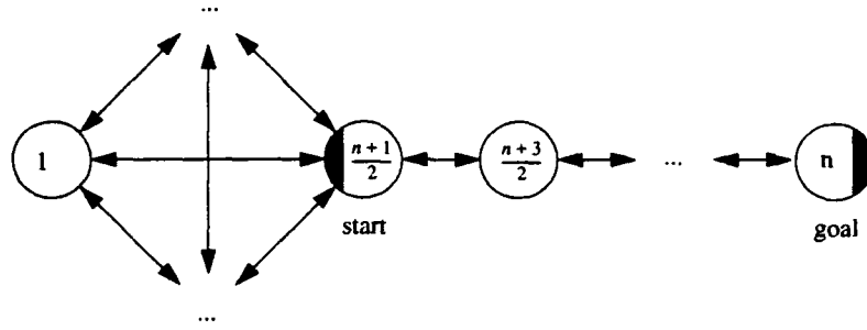
Figure 17: A domain for which a random walk needs 1/8n^3 + 1/8n^2 - 5/8n + 3/8 steps on average to reach the goal state (for odd n \geq 1 ) and for which an admissible, zero-initialized Q-learning algorithm can need at least 1/16n^3 + 3/8n^2 - 3/16n - 1/4 steps to reach the goal state (for n \geq 1 with n \bmod 4 = 1 )
