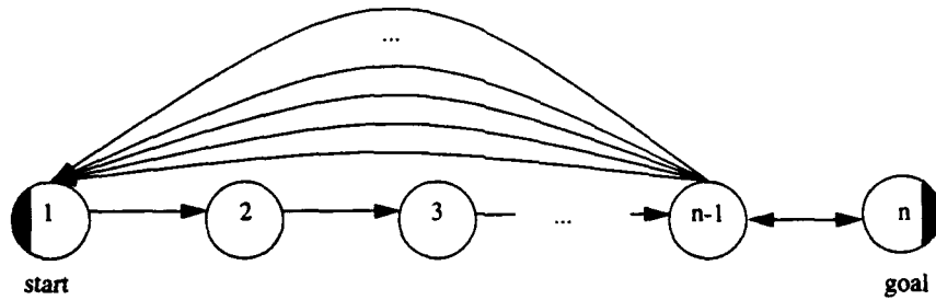
Figure 11: A domain for which an admissible, zero-initialized Q-learning algorithm (and every other uninformed on-line search algorithm) can need at least (e - n + 1)(n - 1) steps to reach the goal state (for n \geq 2 and e \geq n )
