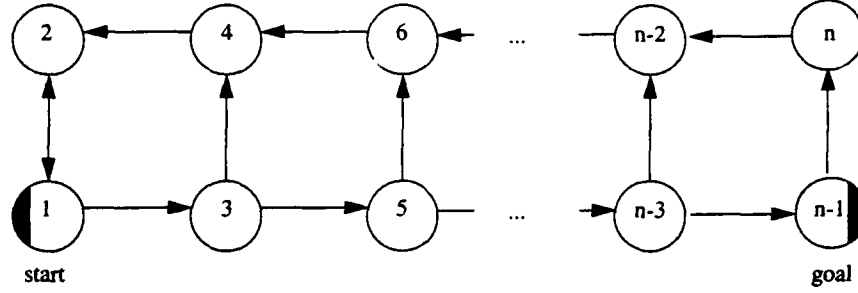
Figure 25: A domain for which an admissible, zero-initialized value-iteration algorithm (and every other algorithm that has to enter a state at least once before it knows the successor states) can need at least 1/4n^2 - 1 steps to reach the goal state (for even n > 1 )
