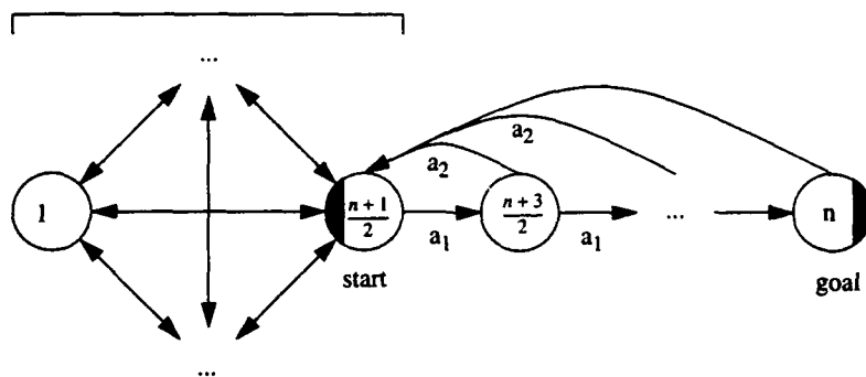
Figure 12: A domain for which an admissible, zero-initialized Q-learning algorithm can need at least 1/16n^3 - 3/16n^2 - 1/16n + 3/16 steps to reach the goal state, but Q_{map} -learning needs only at most 3/8n^2 + 3/2n - 23/8 steps (for odd n \geq 3 )
