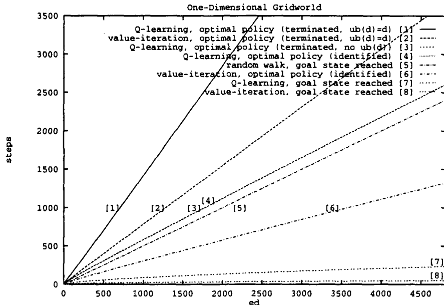
Figure 29: Run-times in the one-dimensional gridworld (as a function of ed = \epsilon(n-1) )
