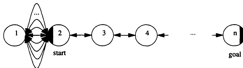
Figure 19: A domain for which every uninformed on-line search algorithm can need at least e + n - 4 steps to reach the goal state (for n > 2 and e \geq 2n - 2 ) and for which an admissible, zero-initialized Q-learning algorithm can need at least 1/2en - 1/4n^2 - 1/2n + 2 steps to reach the goal state (for even n > 2 and e \geq 2n - 2 )
