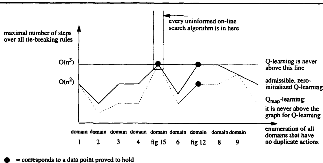
Figure 13: A diagram showing the relationships between an admissible, zero-initialized Q-learning algorithm, the Q_{map} -learning algorithm, and uninformed on-line search algorithms in general (data points for domains other than the ones shown in Figures 12 and 15 are fictitious)
