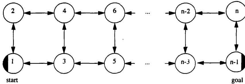
Figure 24: A domain for which an admissible, zero-initialized value-iteration algorithm can need at least 3/16n^2 - 3/4 steps to reach the goal state (for n \geq 1 with n \bmod 4 = 2 )
