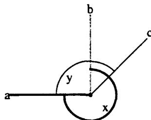
Figure 5-11: Proposed labeling for Figure 5-10.
