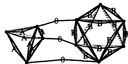
Figure 2-5h: Before solving the coincidence constraints.
