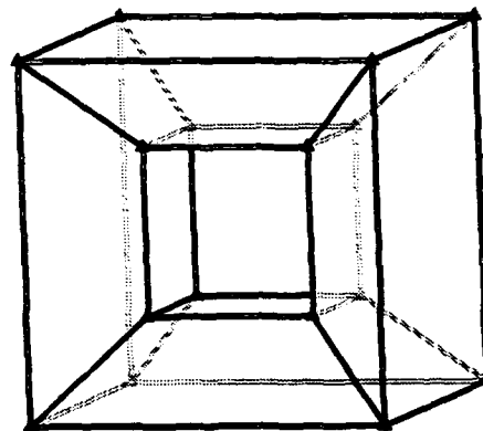
Figure 1-3b: "Tesseract" (16 vertices).
