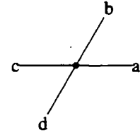
Figure 5-12j: X. ( \angle ca = 180^\circ \wedge \angle bd = 180^\circ )
