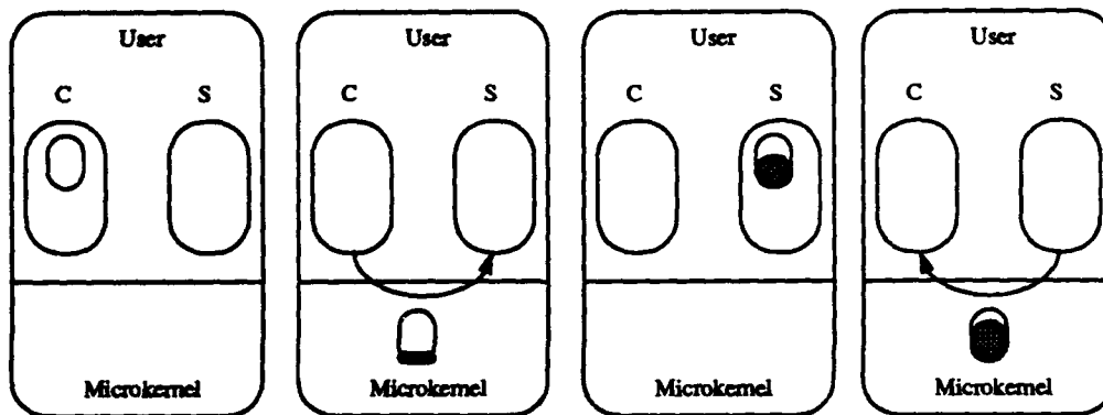
Figure 2: Simple Microkernel Accounting
