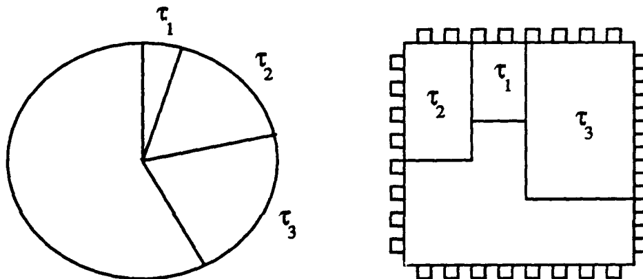
Figure 3: Processor Capacity Reservation
