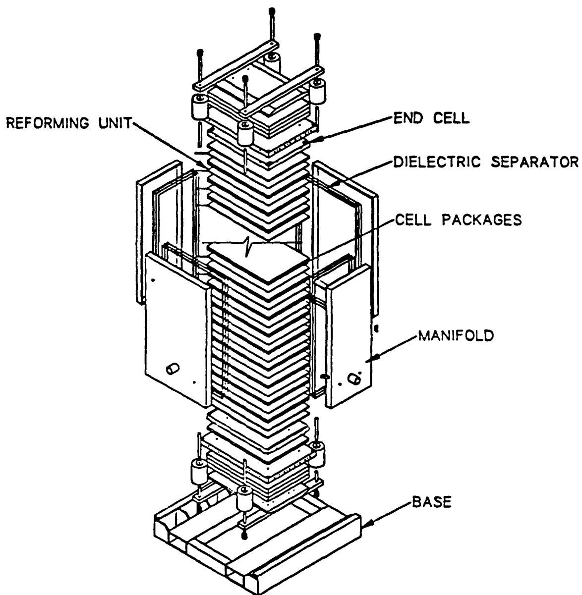
FIGURE 1 DFC STACK ASSEMBLY
