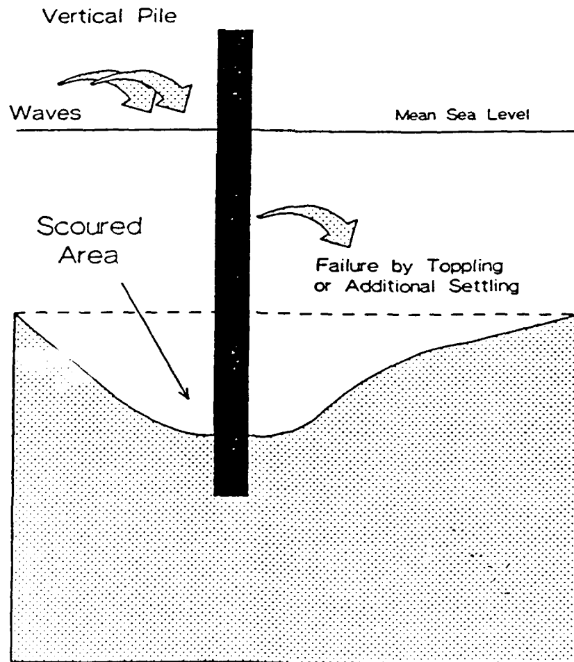
Figure 7. Scour problems at vertical piles
