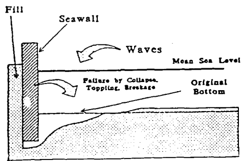
Figure 8. Scour problems at vertical seawalls
