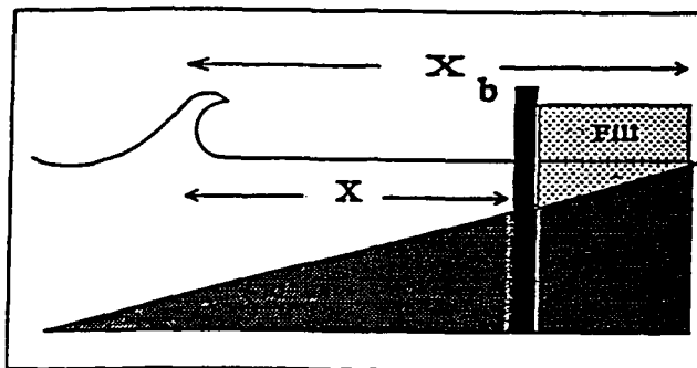
Figure 14. Definition sketch for Jones' method
