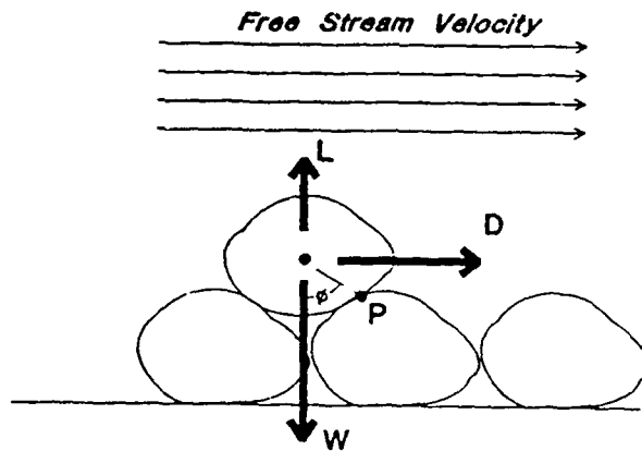
Figure 1. Forces on a particle in unidirectional flows
