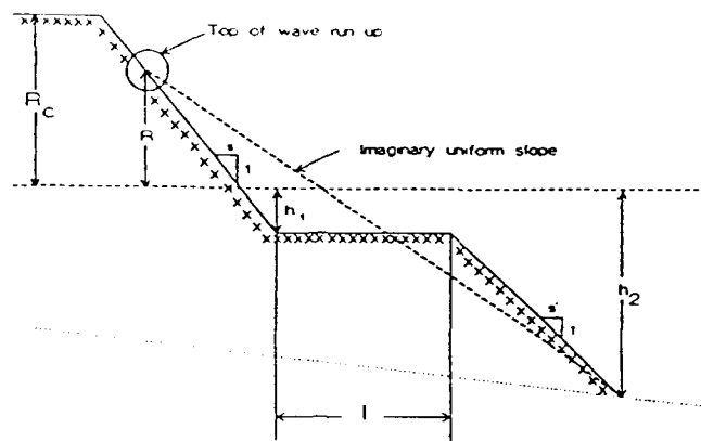
Figure 10. Composite cross-section proposed by Sawaragi (1966)
