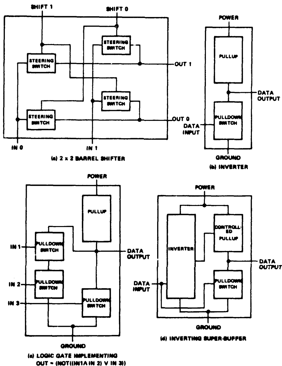
Figure 2. Examples of CSG composite components.
