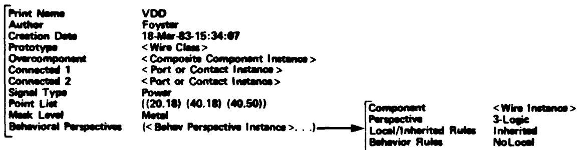
Figure 11. Wire instance object.
