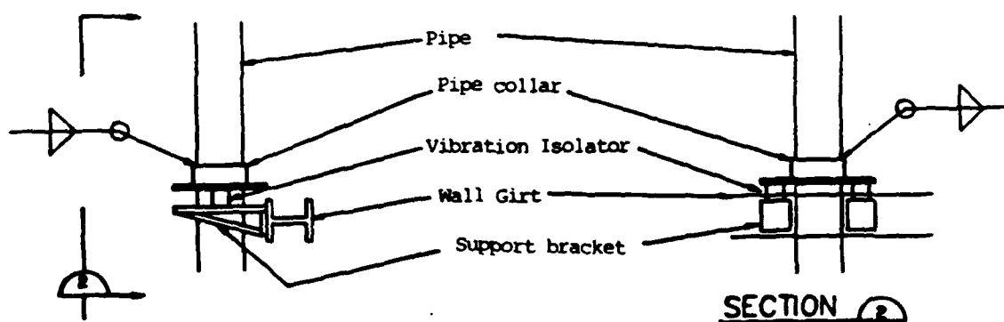
Figure 50. Vertical pipe support and isolation.
