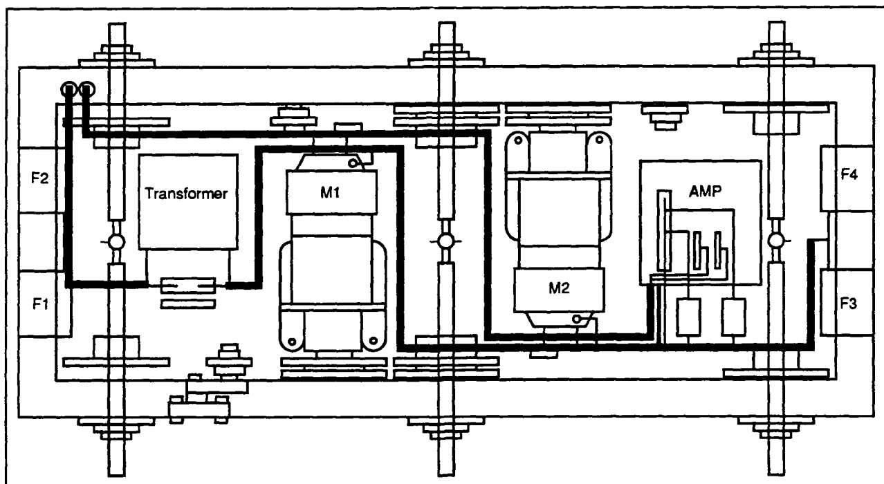
Figure 4-6 Base frame mechanical layout and cabling layout
