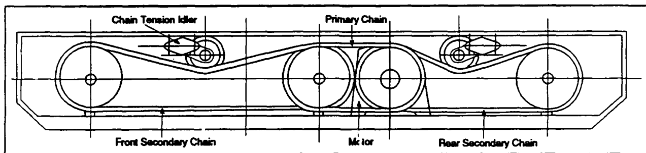
Figure 4-4 Axle Assembly
