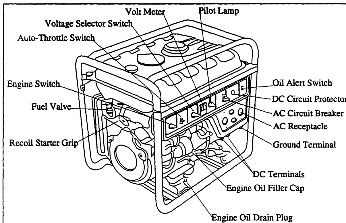
Figure 4-8 Power Generator
