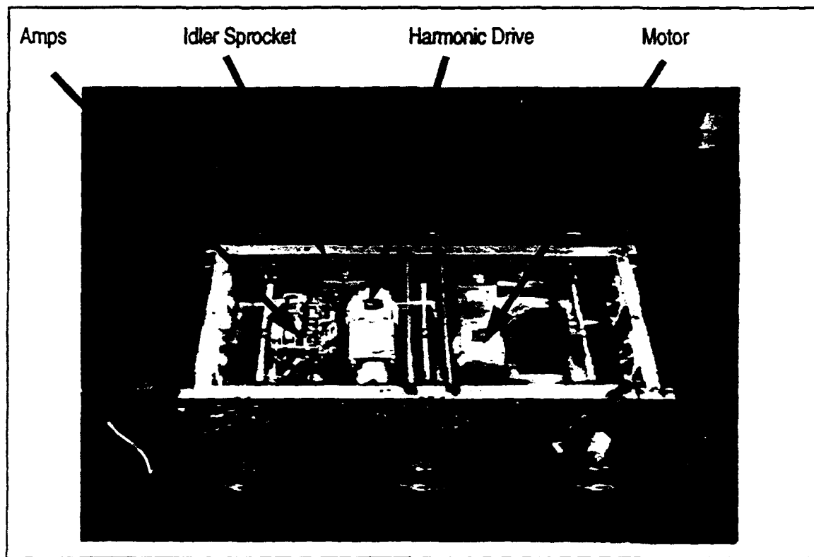
Figure 4-3 Terregator base frame and interior components.
