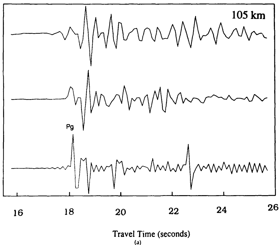
FIG. 7. (a to e) Comparison of observed seismograms (top) with reflectivity synthetic seismograms at 105, 156, 197, 257, and 301 km distance for our final model (middle) and the Leith model (bottom). The amplitude scale is arbitrary.
