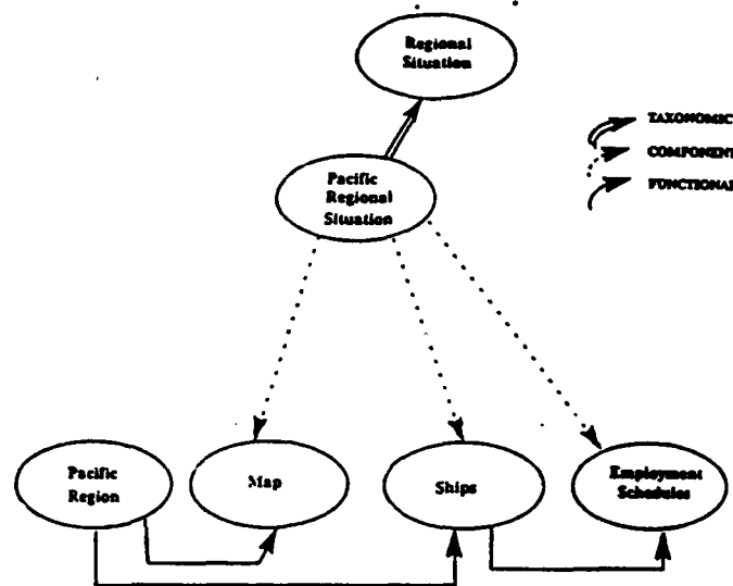
Figure 2: Fragment of Domain Model Containing Pacific Regional Situation .
