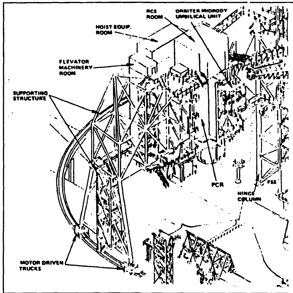
Figure 2.2: Detailed View of Rotating Service Structure (RSS) and the Payload Changeout Room (PCR)
