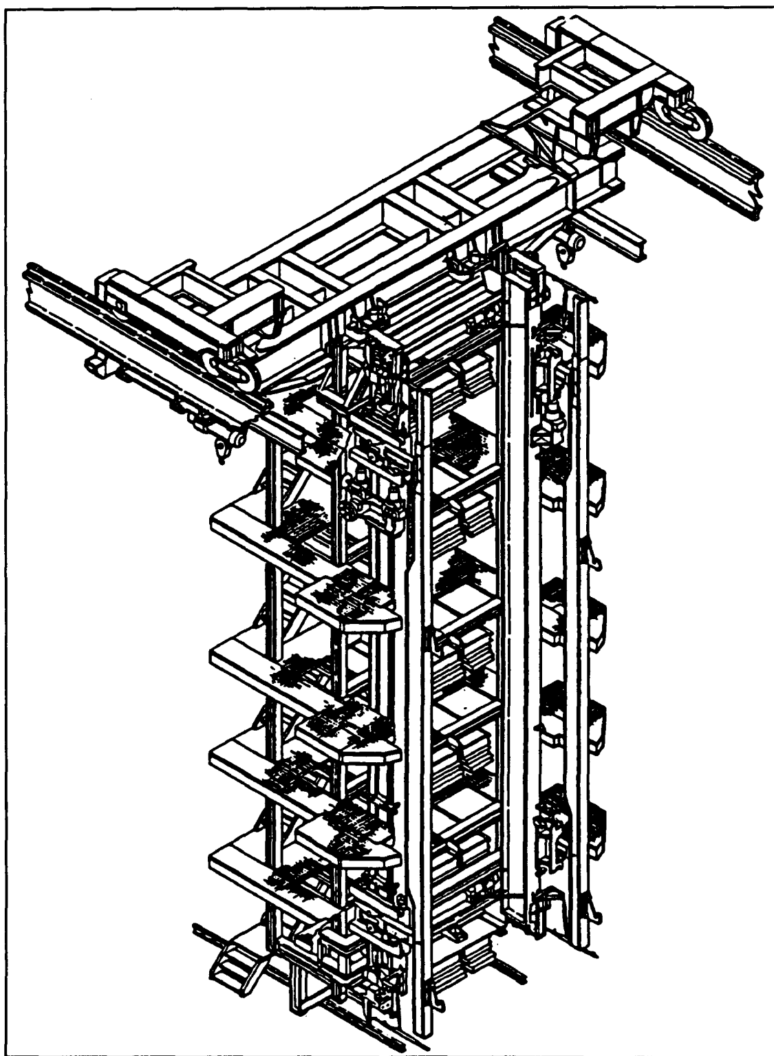
Figure 4: Elevated View of the platform and PGHM systems
