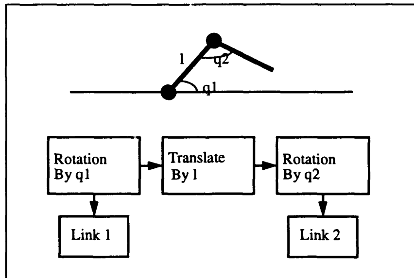
Figure 3.4: Kinematic Model for a 2 DOF serial manipulator
