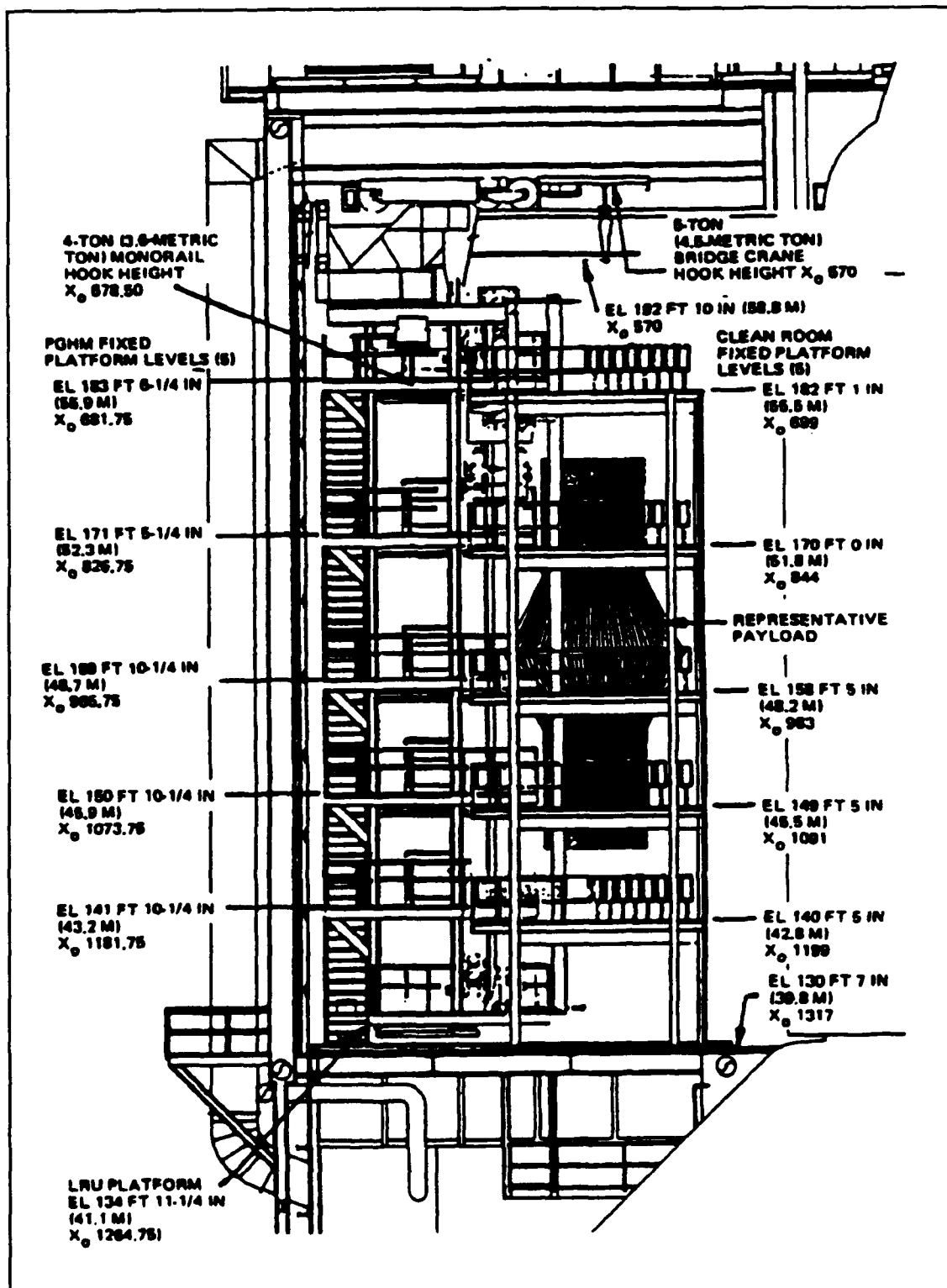
Figure 3: Structure of the platforms and the PGHM inside the PCR, used to access and transport payloads, respectively
