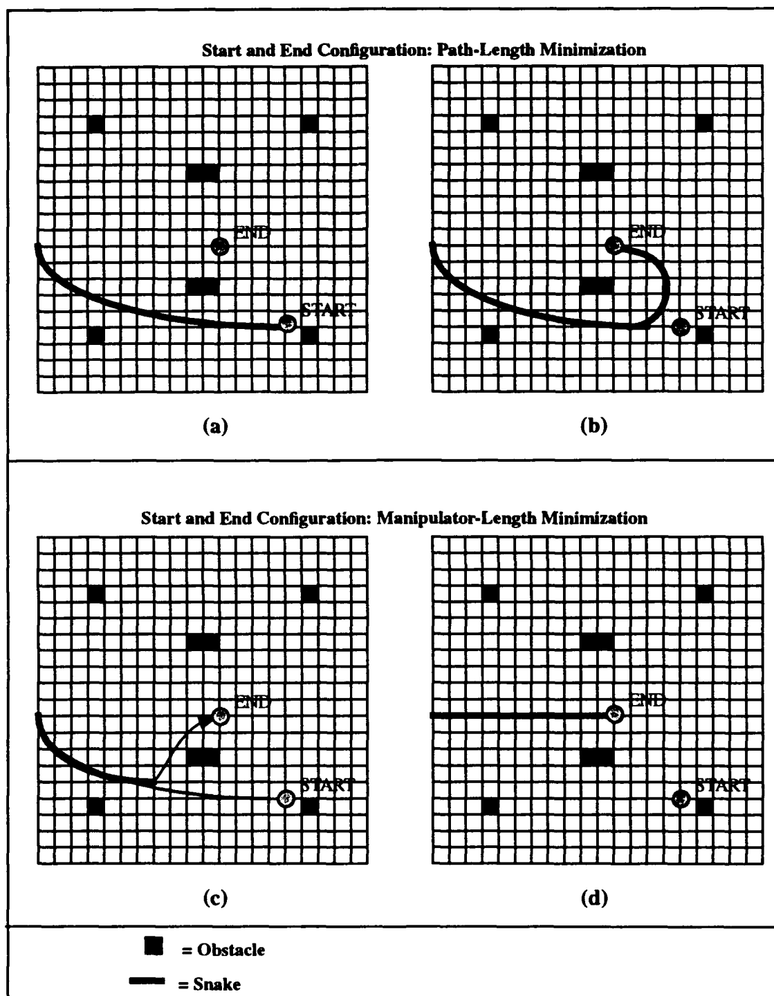
Figure 3.2: Two ways of moving to a new goal
