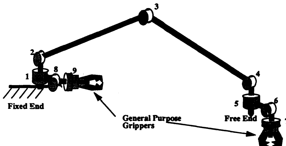
Figure 1: Concept picture of the symmetric robot, SM^2 . While one end is attached to the trusswork fixing joints 8 and 9, the remaining joints 1-7 provide a 7-DOF manipulator configuration.
