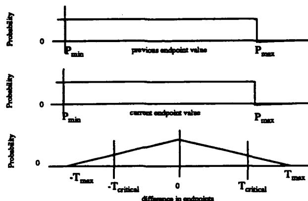
Figure 6: Example of relative probability distribution of two discrete parameter endpoints and probability distribution of the difference of the two parameter endpoints.
