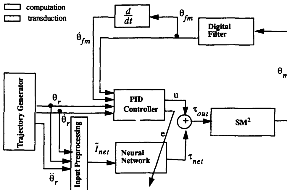
Figure 4: Block diagram of control flow for SM^2 using a neural network. \theta_m , \theta_{fm} , and \theta_r represent the measure joint angle position, the filtered measure joint angle position, and the reference joint angle position respectively. u and e represent the PID feedback signal used for motor control and the PD feedback signal used to correct the network. \tau_{net} , and \tau_{out} represent the output torque value of the network and the composite torque to be sent to the joint. I_{net} represents the input vector to the neural network produced by the preprocessing step (i.e. normalizing and subcomponent composition).
