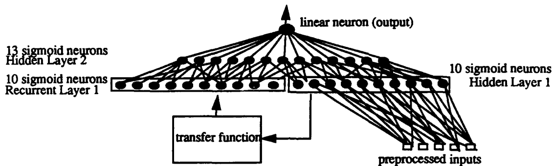
Figure 8: The new neural network architecture used for each of the three joint in Experiment II. Note the first hidden layer is composed of two halves. The activations of the right half (black neurons) are determined as before, but the activations of the left half (gray neurons) are determined by individually applying a transfer function to neurons of the right half. Note that each level is fully connected.
