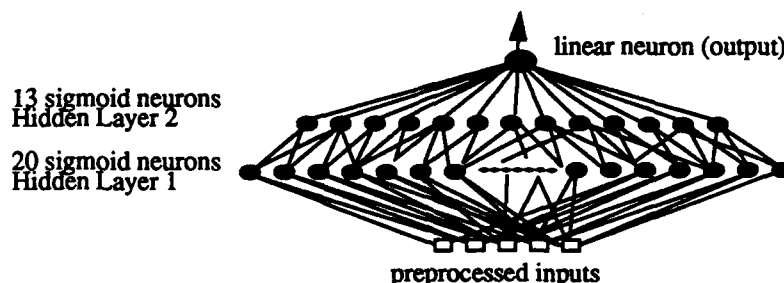
Figure 7: The neural network architecture used for each of the three joint in Experiment I. Each layer is fully connected.
