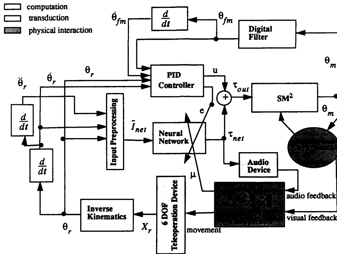
Figure 11: Block diagram of control flow for SM 2 using teleoperation. X_r represents the Cartesian reference frame as received from the 6DOF device. \mu represents the learning rate which is now controlled by the teleoperator. The other symbols are defined as previously shown in Figure 4.
