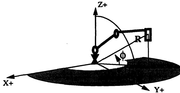
Figure 5: The representation of polar coordinates defined by \theta , \phi , and R . Each parameter has a selected minimum and maximum. For SM^2 , the workspace defined by the limits forms a quartersphere with a hollow center.
