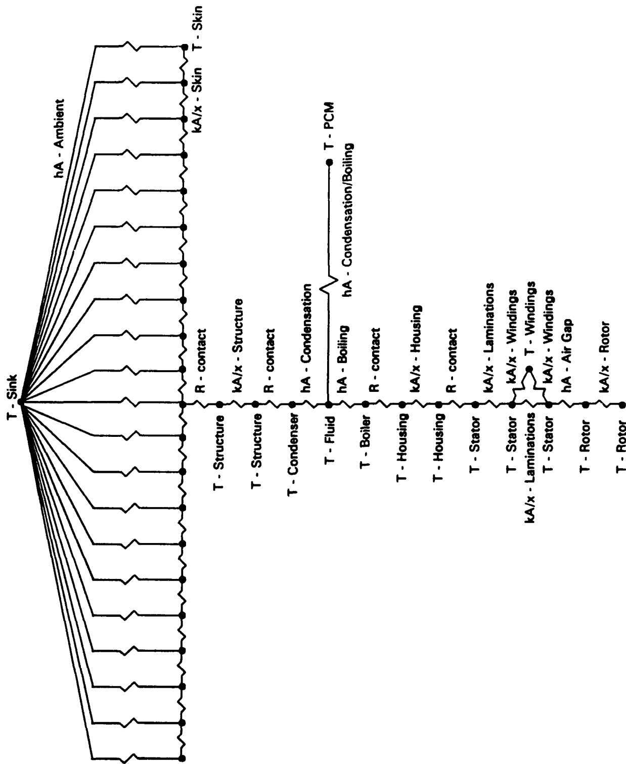
Figure 4.2 SINDA Model Schematic
