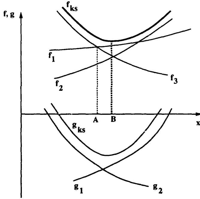
Figure 1: KS Function for Objectives and Constraints
