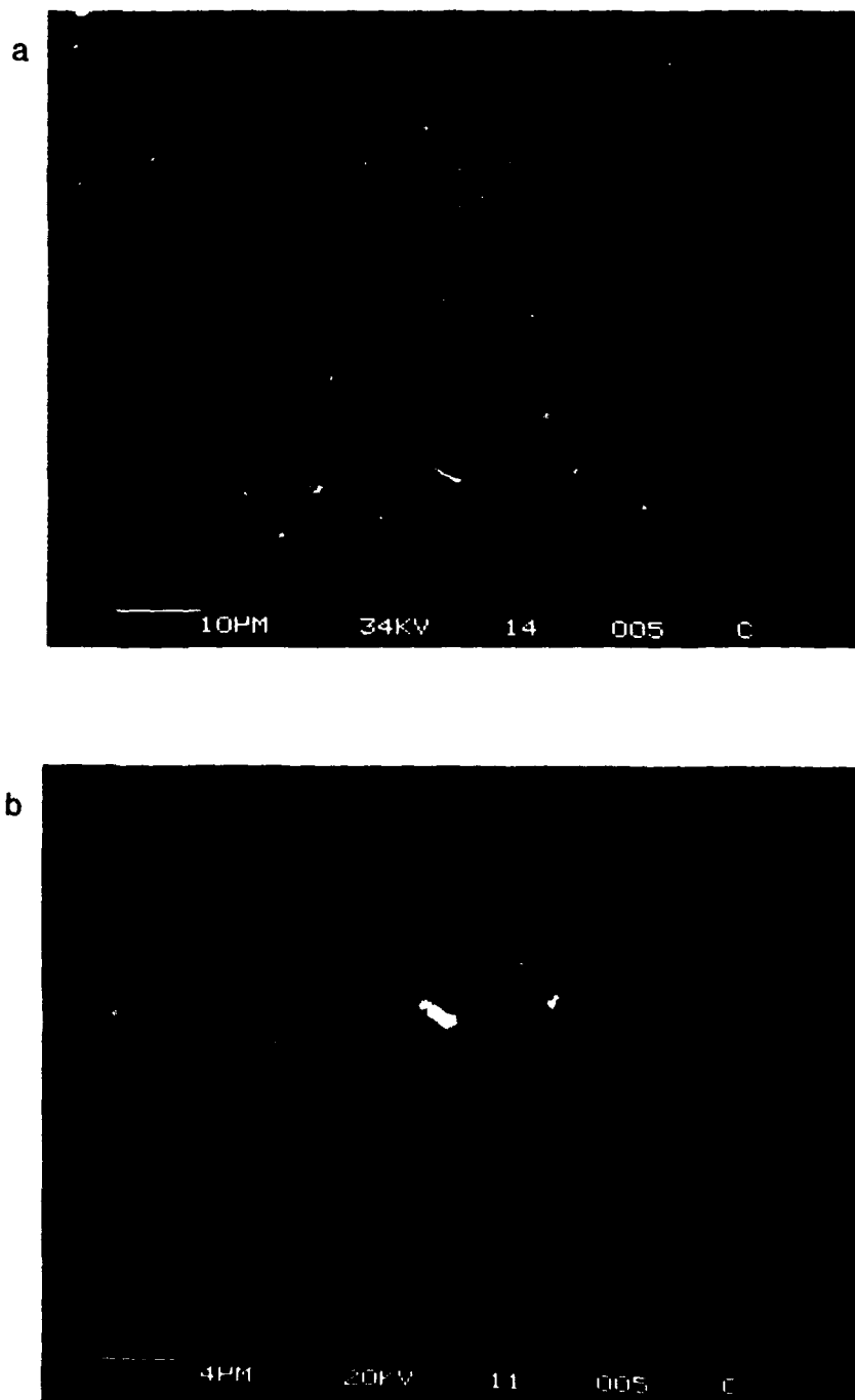
Figure 3: Scanning electron micrographs (backscatter image) of coarse alloy carbonytrides in as-received BIS 812 EMA steel.
