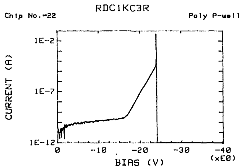
Figure 12. An example of measured and stored VROB data.
