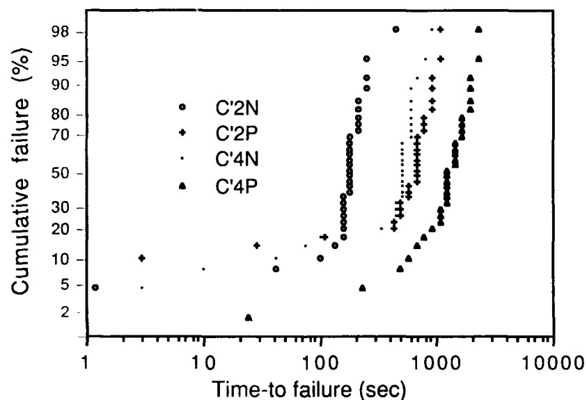
Figure 16. The TDDDB distributions derived from VROB distributions at 125°C for wafers C'2 and C'4.
