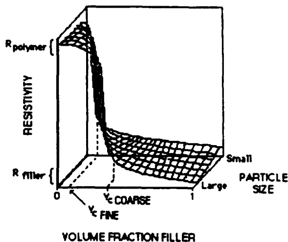
Figure 9: Qualitative representation of the percolation behavior of composites of identical chemical composition but varying particle size.
