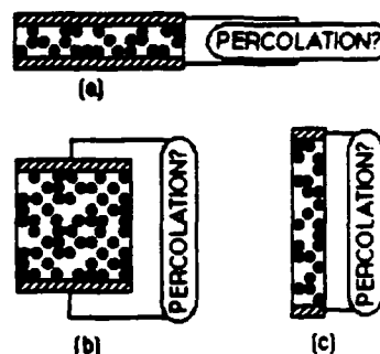
Figure 5: Graphics output from the Monte Carlo percolation simulation for (a) favorable percolation geometry ( G=5.0 ), (b) neutral geometry ( G=1.0 ), and (c) unfavorable percolation geometry ( G=0.2 ).
