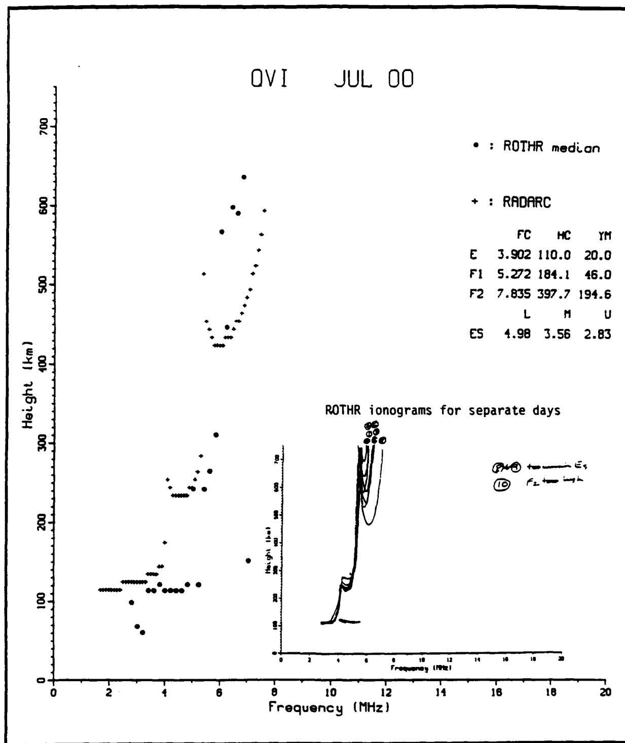
Figure 3.5. RADARC predicted quasi-vertical ionogram for hour 00 UT (local daytime) of July vs. the monthly median of ROTH observed ionograms. The RADARC prediction is based on an estimated monthly median overhead ionosphere. On each individual ROTH ionogram, the trace is taken to be the maximum power over height at each frequency. The median height of all traces is then taken at each frequency. This plot is based on about 40 to 45 ROTH traces or about ten days of data.
