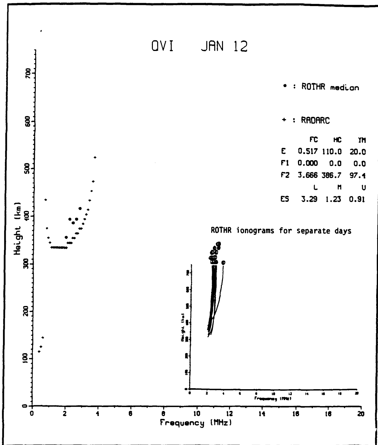
Figure 3.2. RADARC predicted quasi-vertical ionogram for hour 12 UT (local nighttime) of January vs. the monthly median of ROTH observed ionograms. The RADARC prediction is based on an estimated monthly median overhead ionosphere. On each individual ROTH ionogram, the trace is taken to be the maximum power over height at each frequency. The median height of all traces is then taken at each frequency. This plot is based on about 40 to 45 ROTH traces or about ten days of data.
