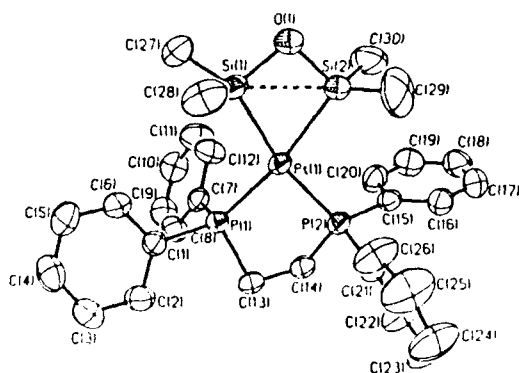
Figure 2. Thermal ellipsoid plot for 9b (50% probability). Hydrogen atoms omitted for clarity.
