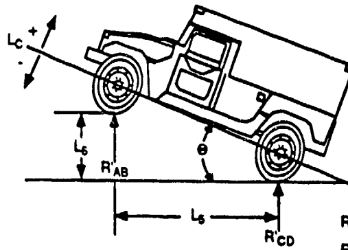
SIDE VIEW INCLINED
