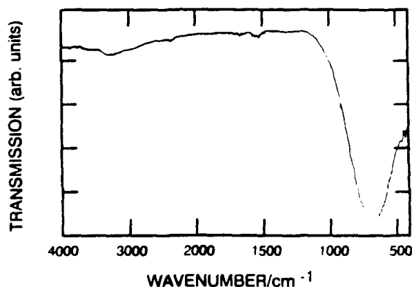
FIG. 2. IR transmittance spectrum of a 1 \mu m thick AlN film grown on a KBr plate.
