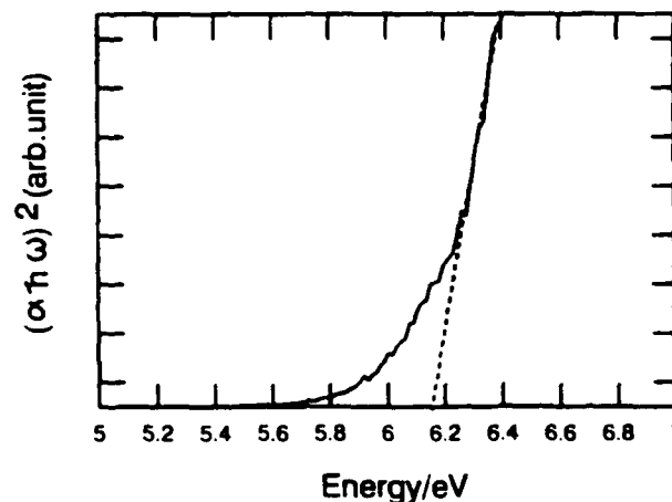
FIG. 4. A plot of the square of (absorbance) \times (photon energy) as a function of photon energy. This was taken from the UV absorption spectrum corrected for surface scattering and reflection.
