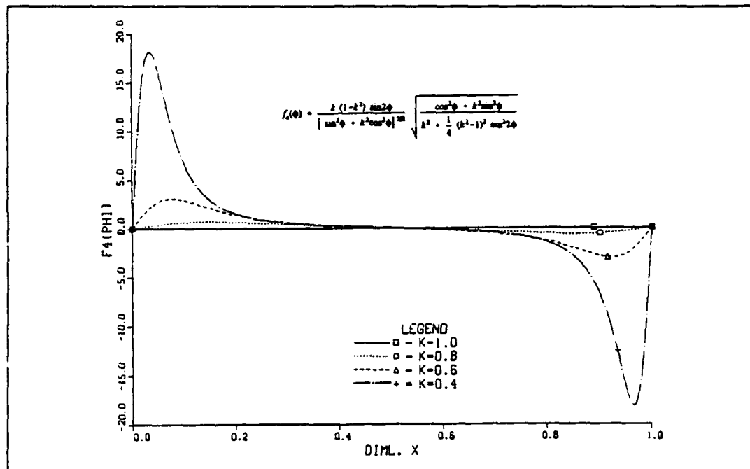
Figure IV-11. Surface Tension Function, f_4(\phi) for Varying Eccentricity.
