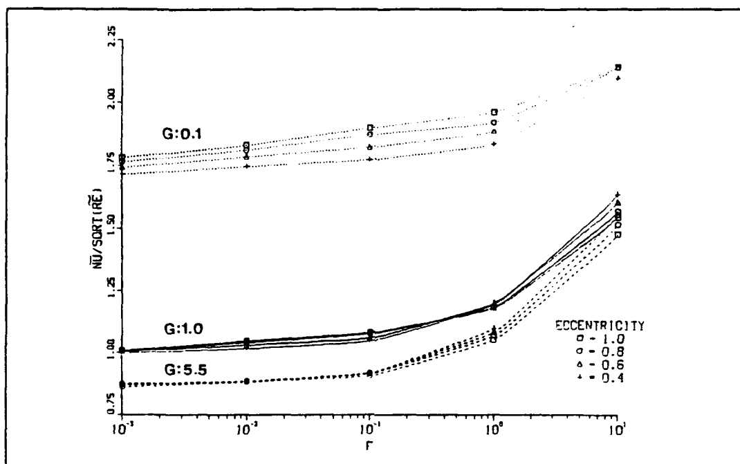
Figure IV-8. Effects of Vapor Velocity and Vapor Separation on Mean Nu using the Two-Phase Boundary-Layer Approximation Analysis Method.
