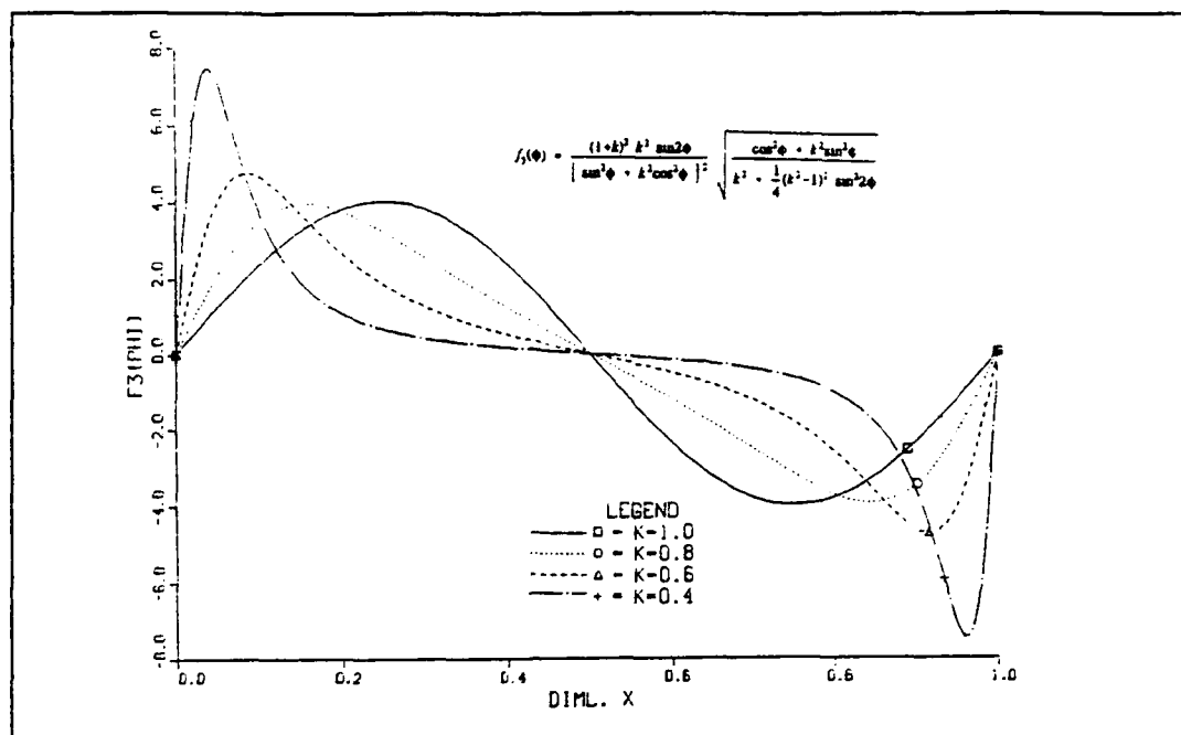
Figure IV-13. Pressure Gradient Function, f_3(\phi) , for Varying Eccentricity.
