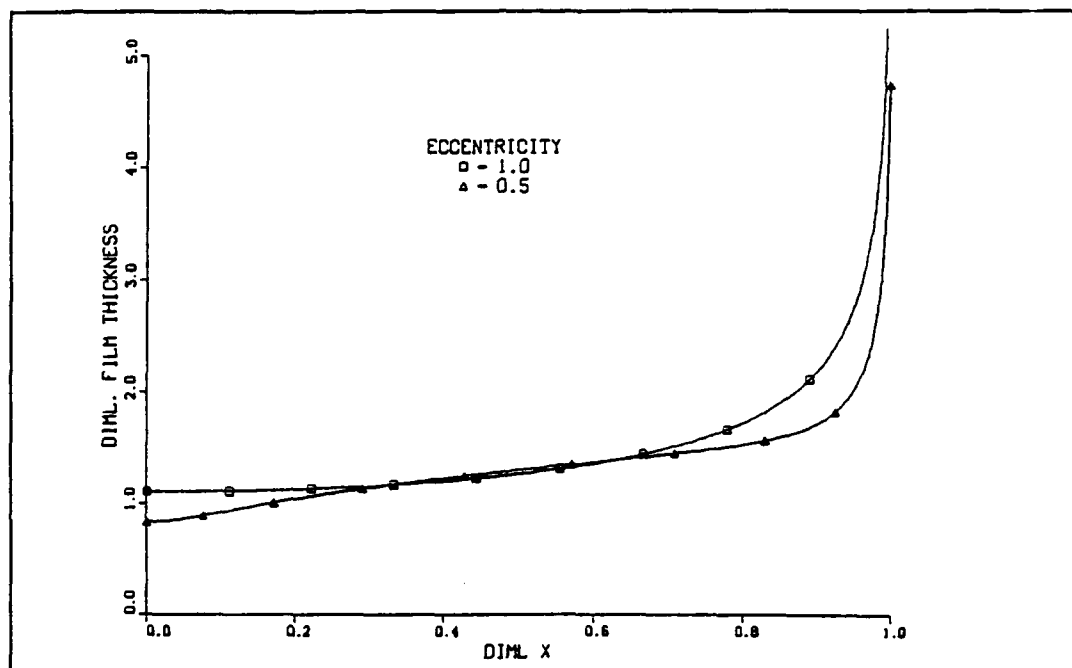
Figure IV-2. Local Film Thickness for Varying Eccentricity ( k ).
