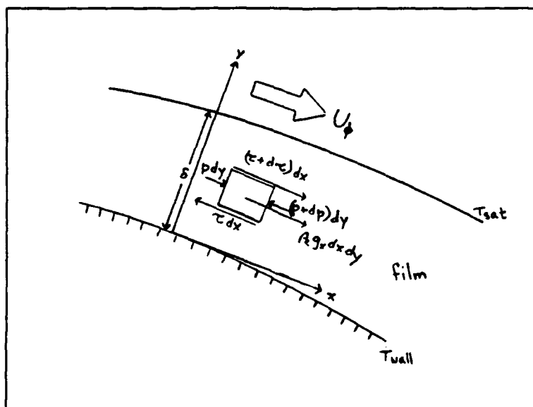
Figure II-5. Condensate Film Element for Mixed Convection with Pressure Gradient.
