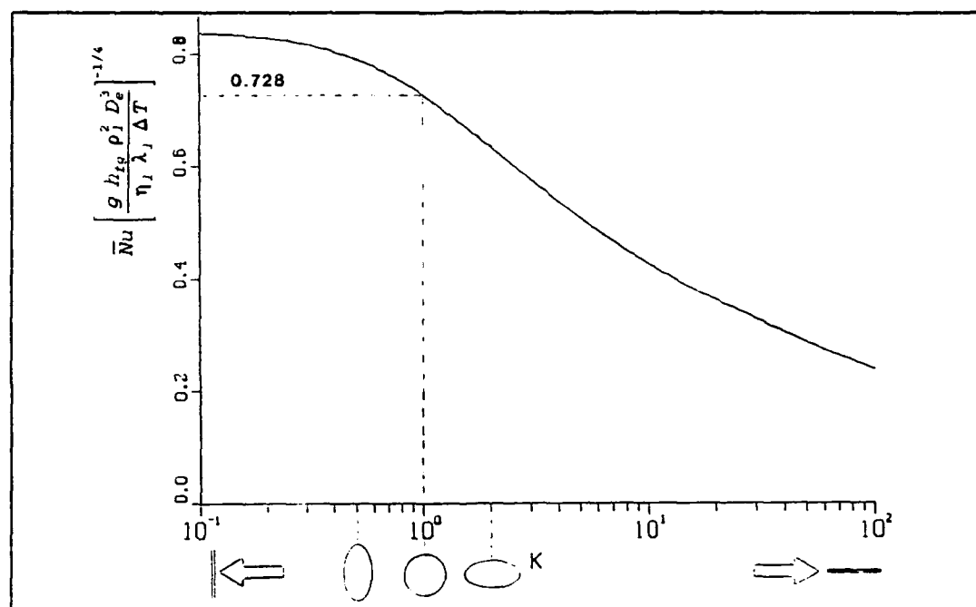
Figure IV-3. Mean Nu Leading Coefficient for Varying k .
