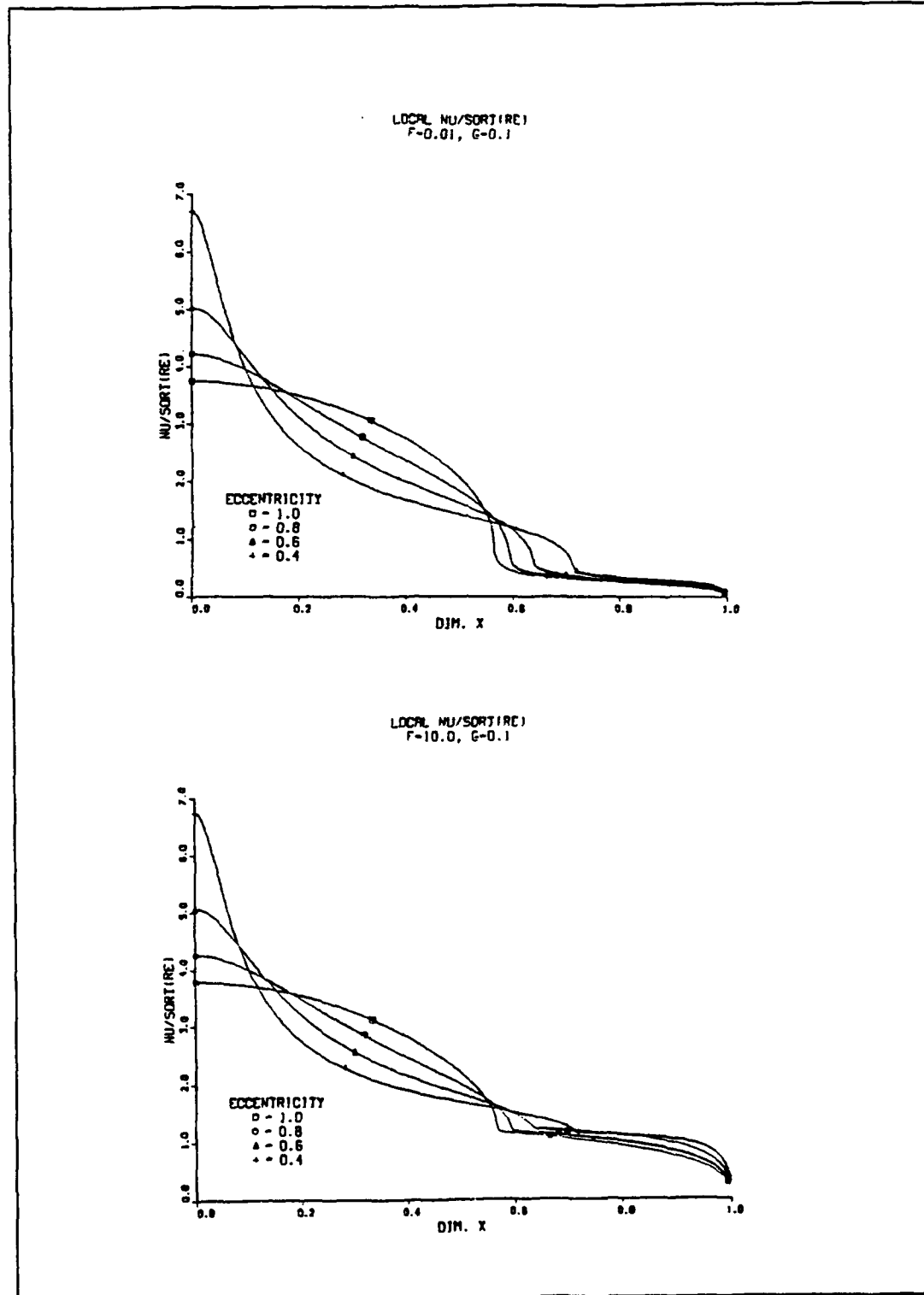
Figure 10 a and b. Local Nu for Varying G , F and k from the Two-Phase Boundary Layer Shear Stress Analysis Method.
