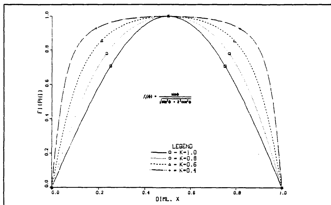
Figure IV-1. Gravity Function, f_1(\phi) vs. Streamwise Length, x .
