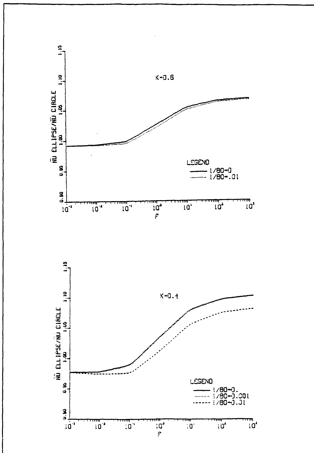
Figure IV-12. Effect of Surface Tension on the Mean Nu for k = 0.4 and 0.6 .
