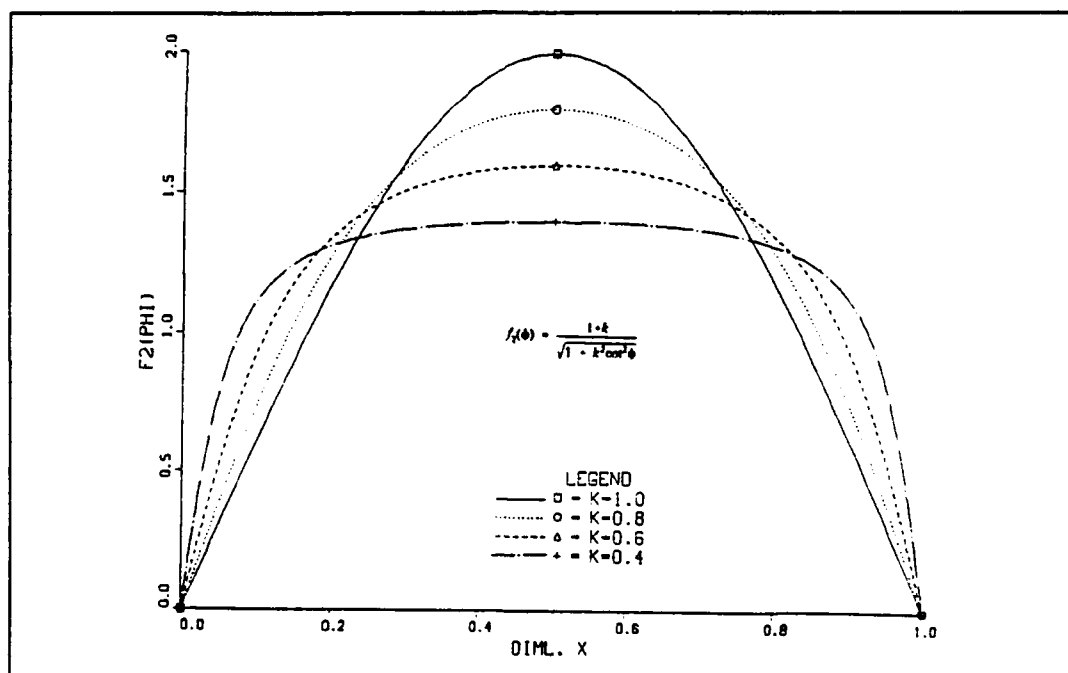
Figure IV-4. Vapor Velocity Function, f_2(\phi) , for Varying k .
