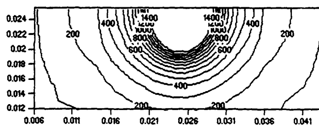
(b) TRAVERSE TEMPERATURE CONTOUR
