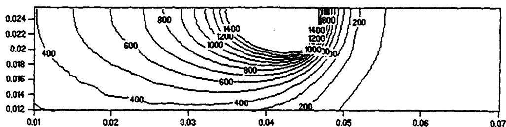
(a) LONGITUDINAL TEMPERATURE CONTOUR
