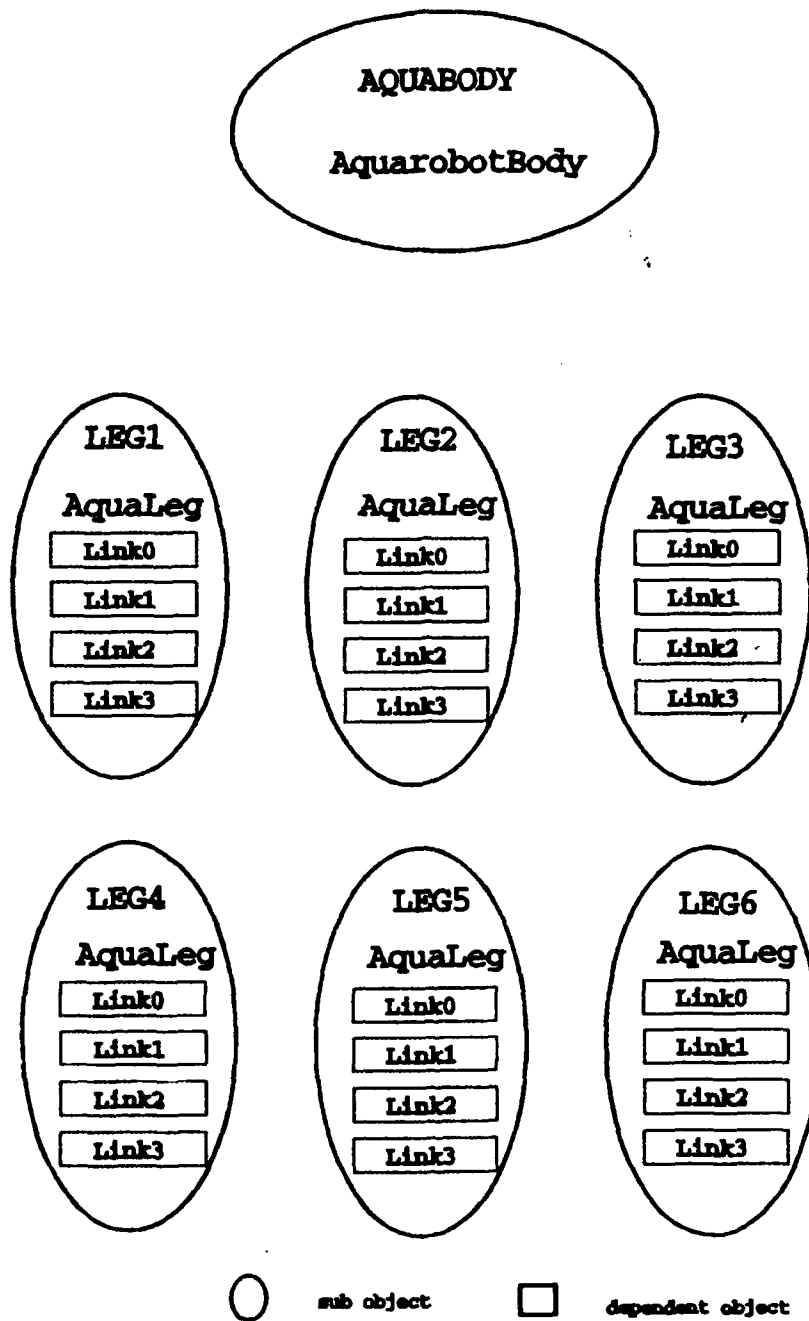
Figure 7.3 C++ Object Hierarchy
