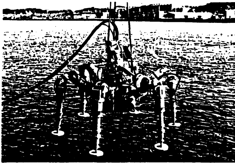
Figure 3.1 Photograph of Aquarobot
