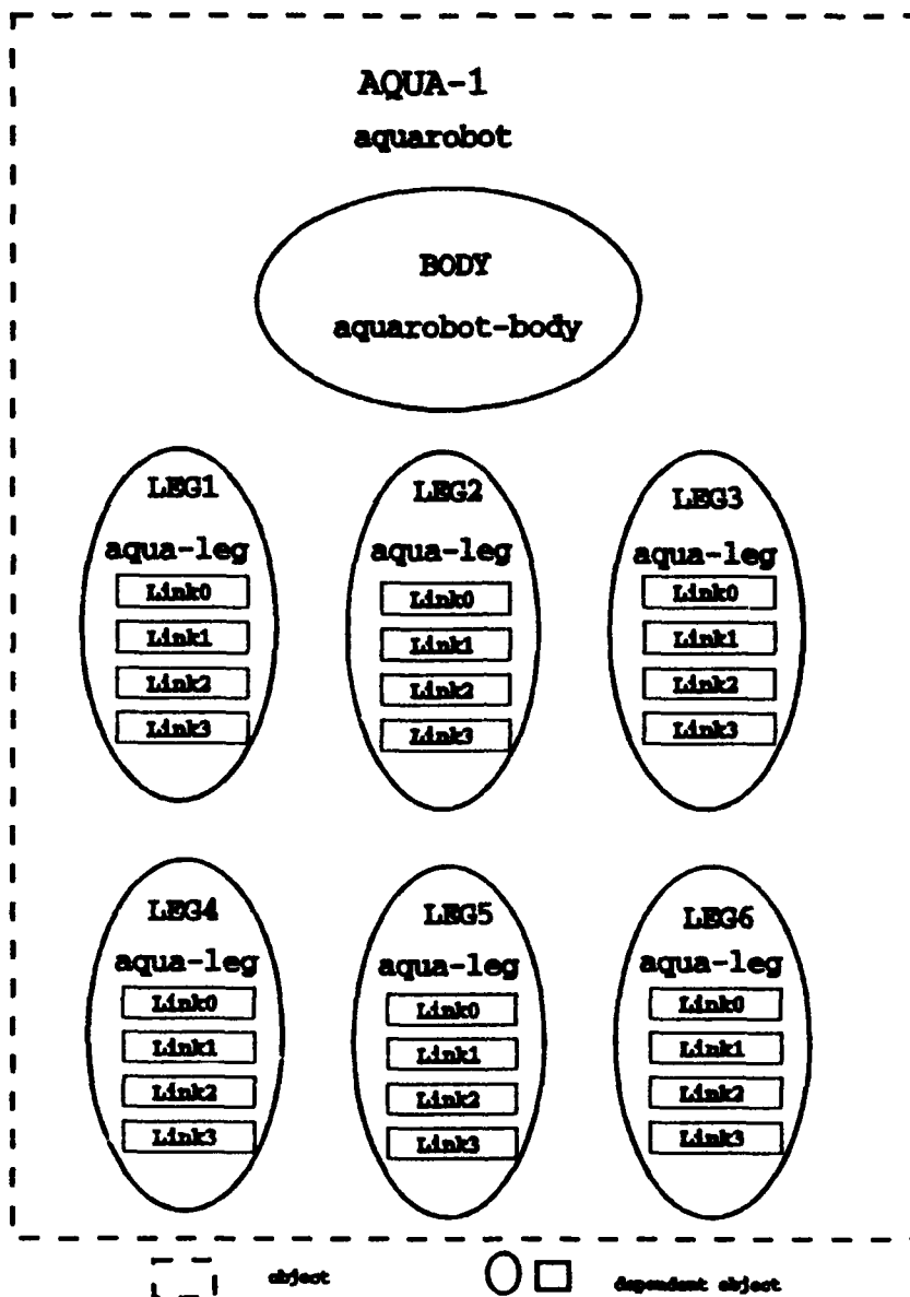
Figure 7.4 CLOS Object Hierarchy
