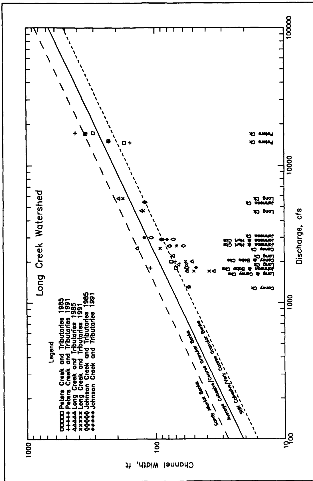
Figure 28. Hydraulic geometry relationships, Long Creek, discharge versus width
