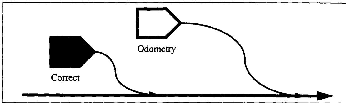
Figure 30: Reset_Rob Function
