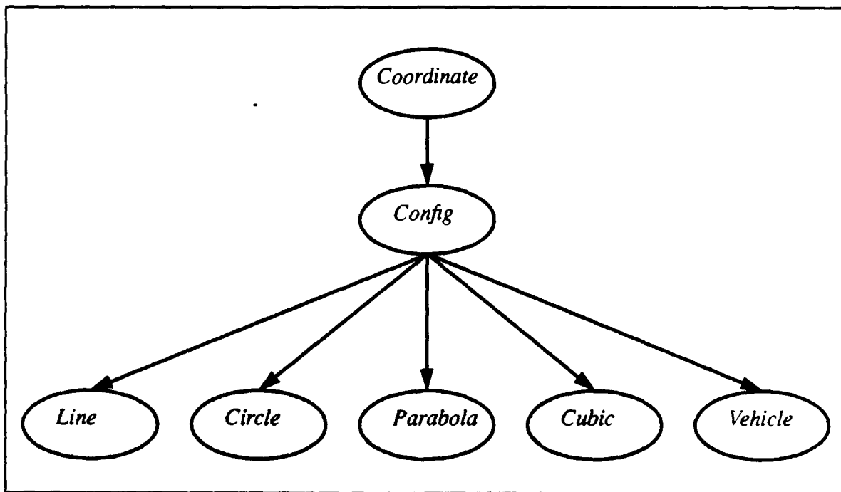
Figure 4: Inheritance Schema
