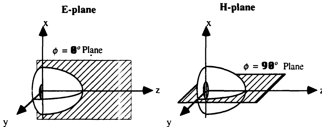
Figure 4.1 Orientation of E-plane and H-plane
