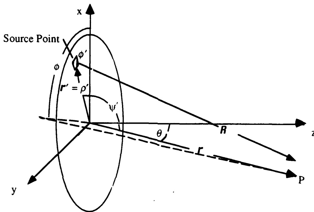
Figure 2.8 Circular Aperture Antenna Source Point
