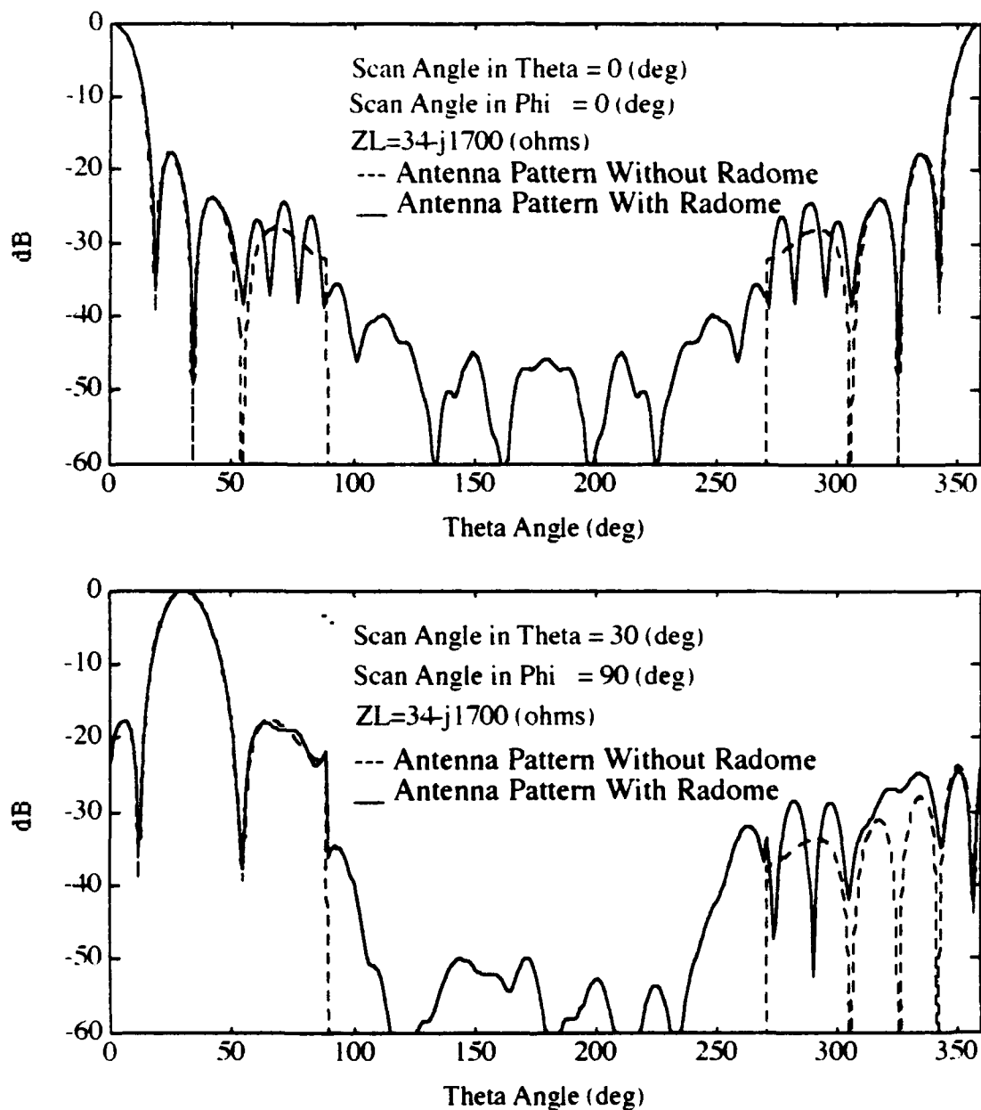
Figure 4.6 H-Plane Pattern of Antenna with an Ogive Radome Z_L = 34 - j1700 \Omega
