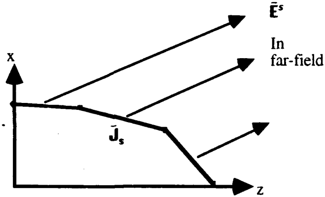
Figure 2.7 Scattered Field
