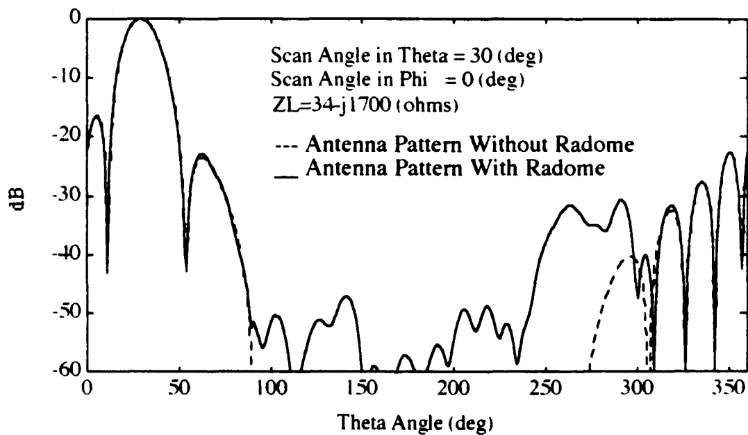
Figure 4.5 E-Plane Pattern of Antenna with an Ogive Radome Z_L = 34 - j1700 \Omega
