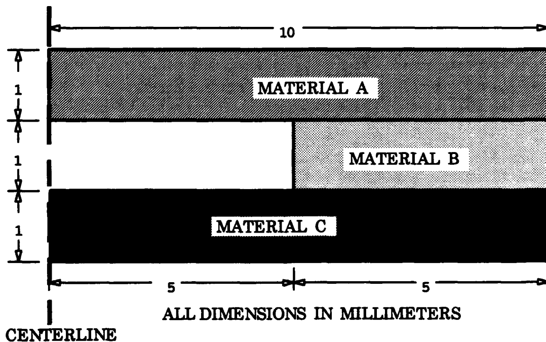
Figure 3.1 Tri-material Configuration
