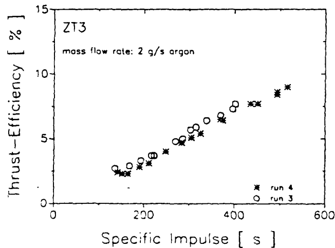
Fig. 3.10: Thrust efficiency as a function of specific impulse of the ZT3-thruster, running with 2 g/s argon
