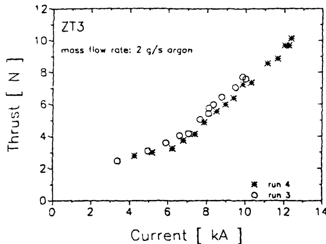
Fig. 3.9: Thrust vs. current curve for the ZT3-thruster, running with 2 g/s argon
