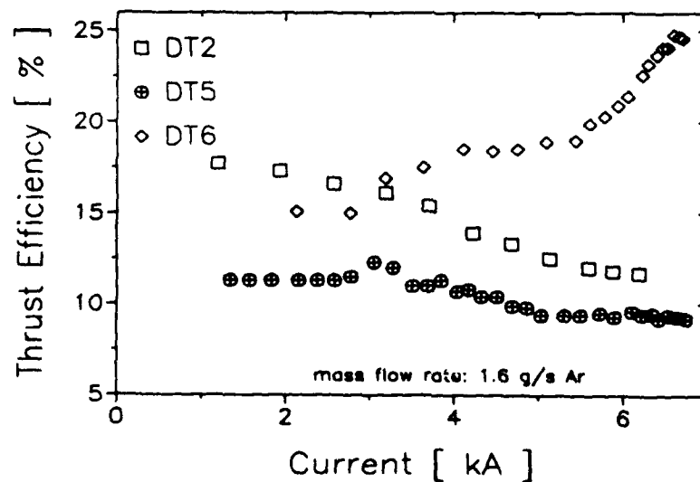
Fig. 2.8: Thrust efficiency vs. current curve of the nozzle type DT-thrusters, running with 1.6 g/s argon. ( DT6 data are preliminary )
