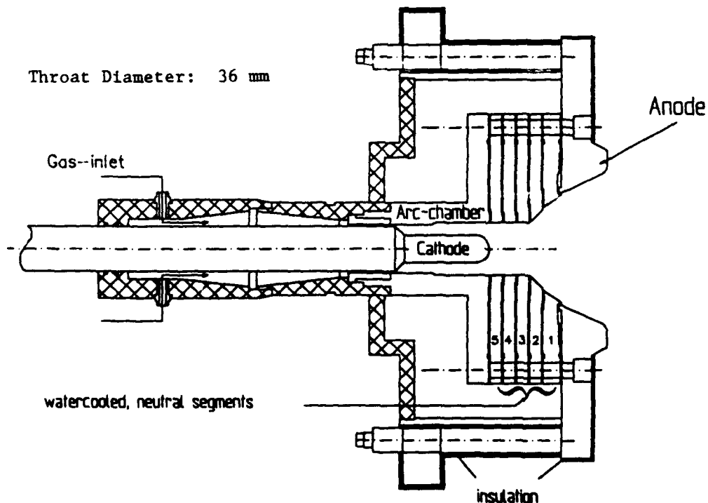
Fig. 2.2: Configuration of the nozzle type MPD-thruster DT6
