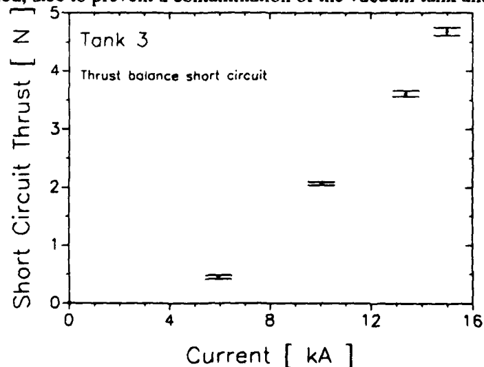
Fig. 3.7: Short Circuit Thrust of the thrust balance for the cylindrical thrusters
