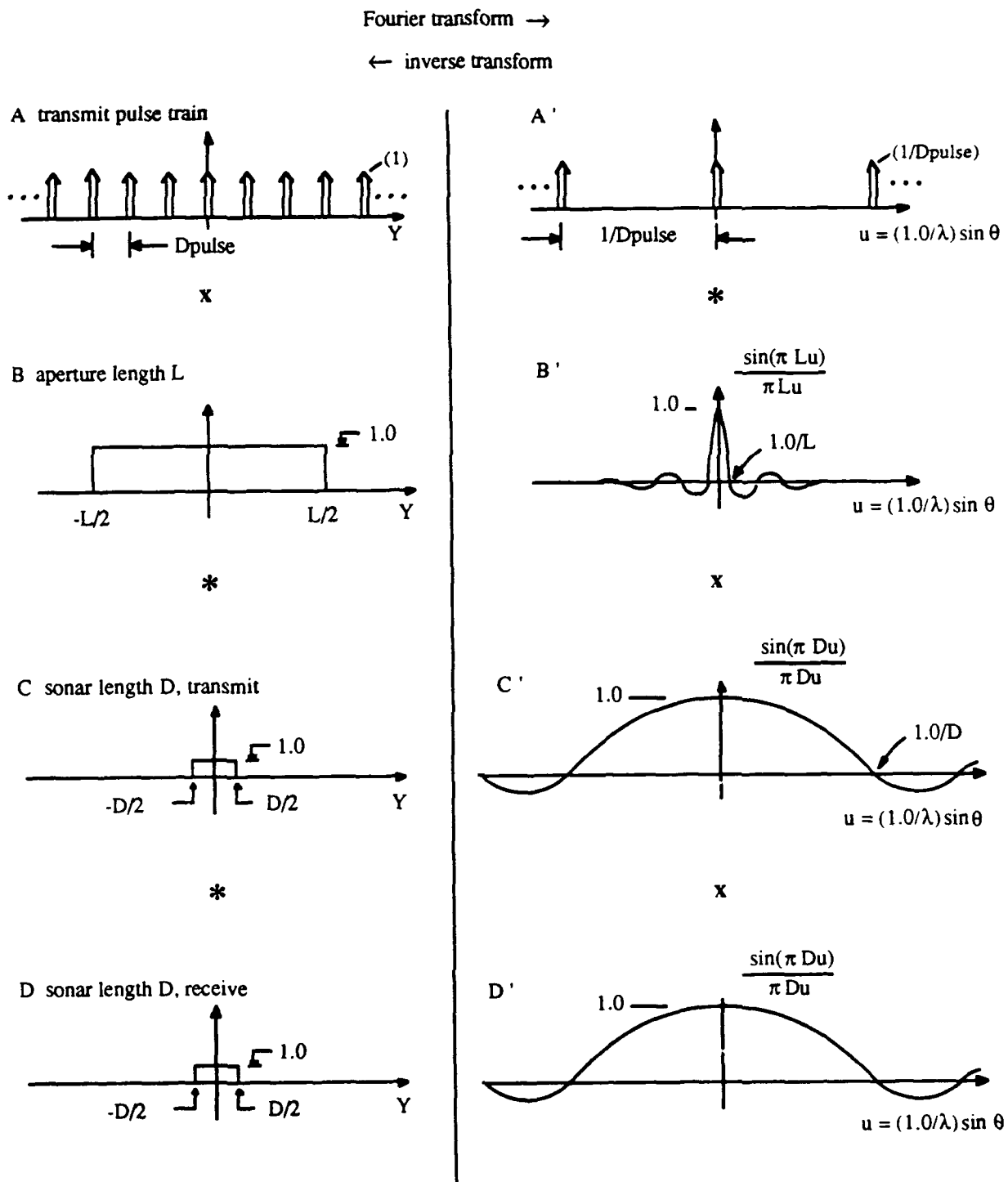
Figure 2.13 - Transform Pair: Geometry and Wavenumber Spectra
