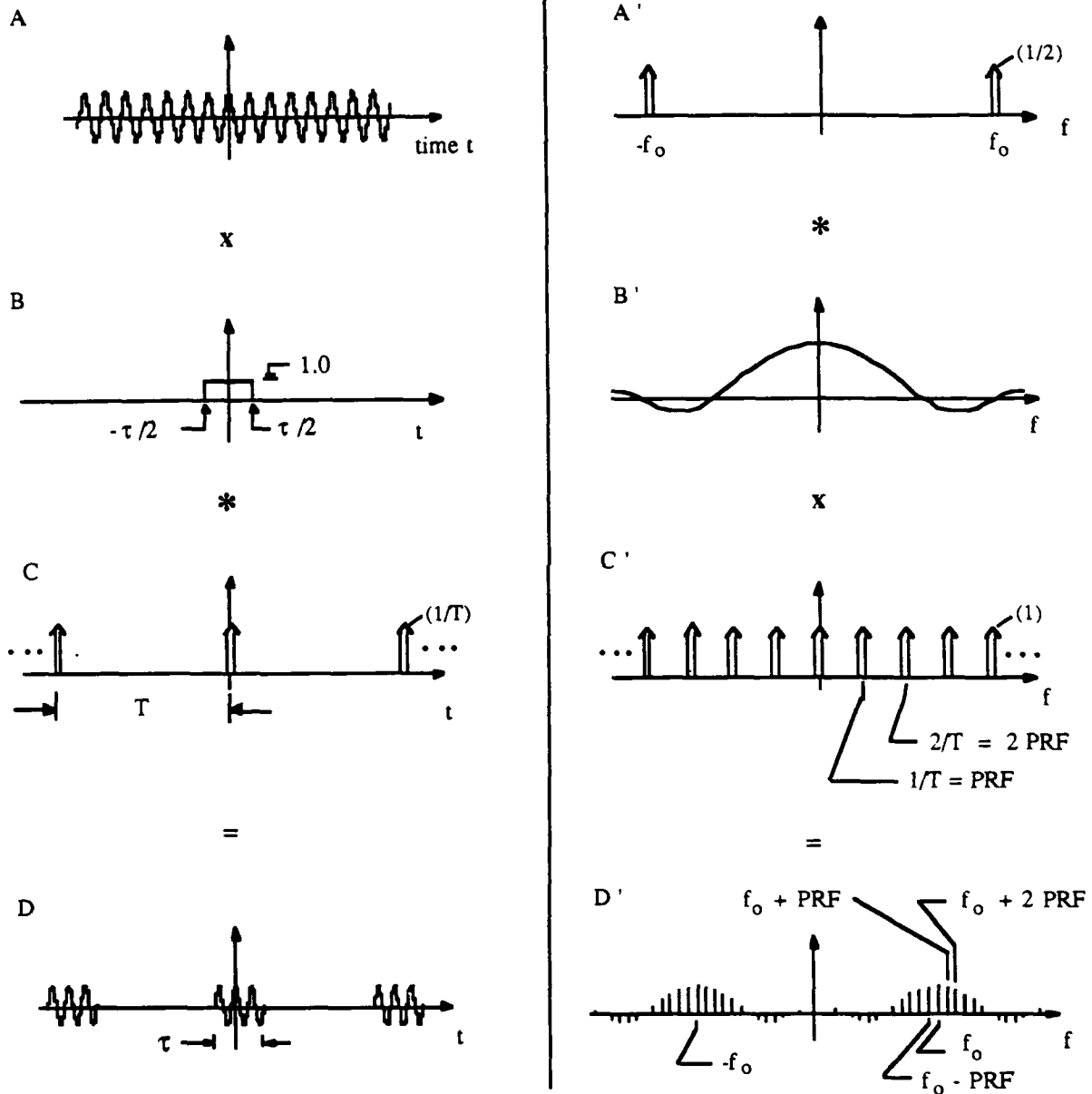
Figure 2.14' - Transform Pair: Transmit Signal and Frequency Spectra
