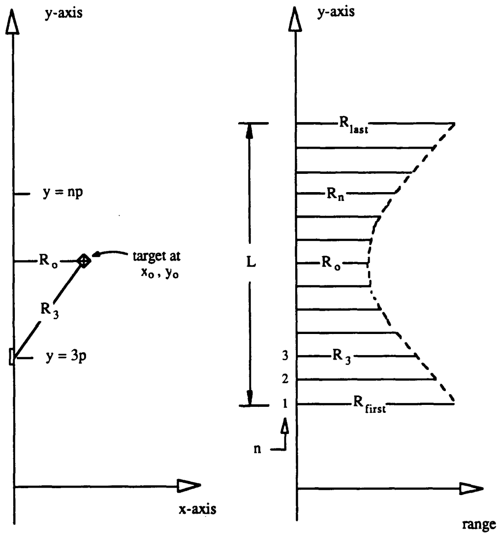
Figure 2.7 - Range Migration Hyperbola of Target at x_o, y_o
