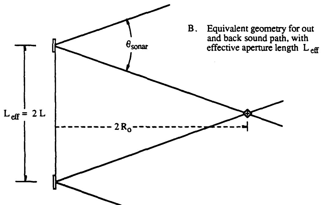
Figure 2.10 - Synthetic Aperture Lengths L and L_{eff}
