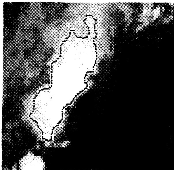
Figure 4: A subframe of GOES imagery taken from 3, with contours overlaid for pixel brightness 181.
