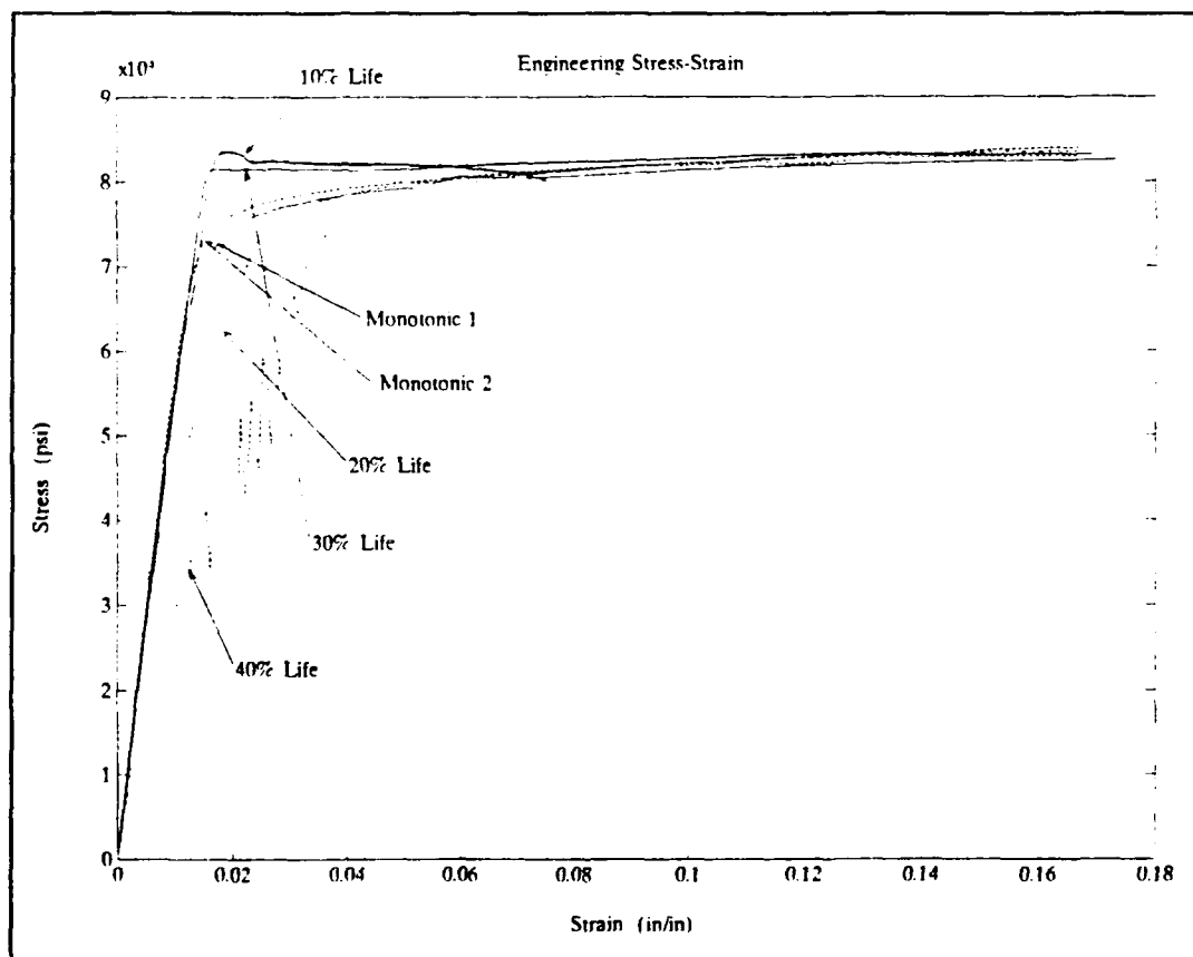
Figure 9 Stress-Strain Curves
