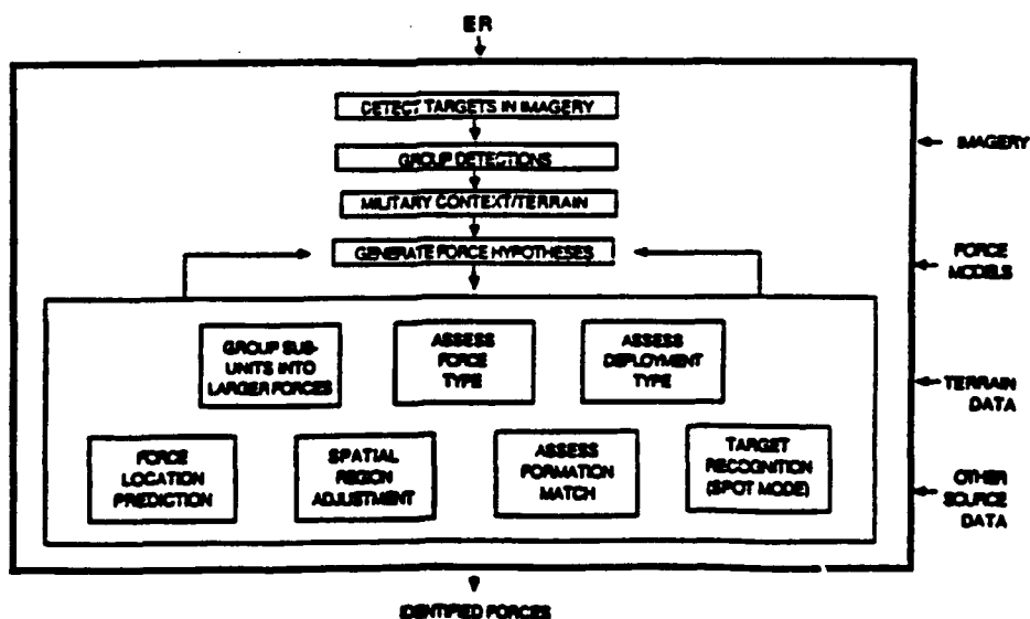
IES/BTI Processing Concept
