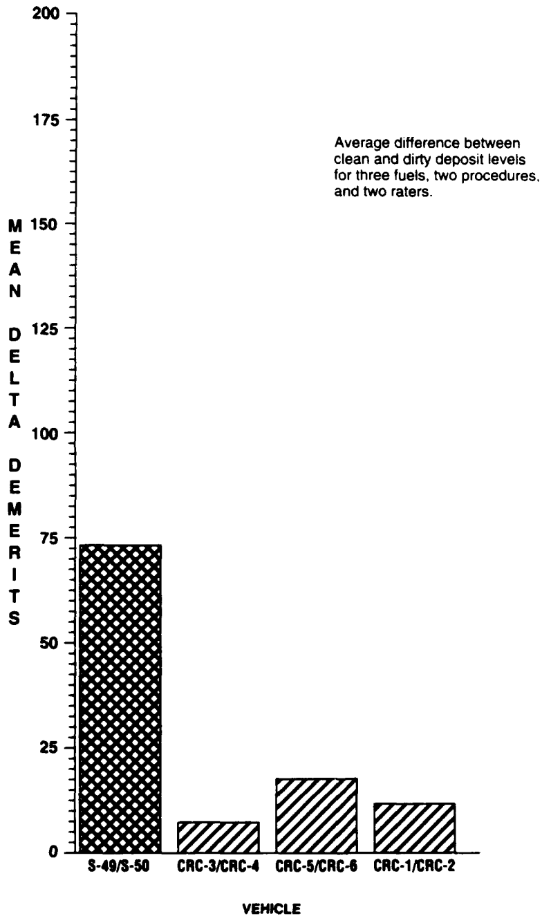
FIGURE 1 INCREASE IN DRIVEABILITY DEMERITS WITH DEPOSITS BY VEHICLE MODEL
