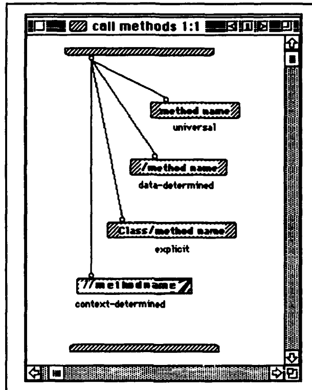
Figure 5: Method Calling Formats
