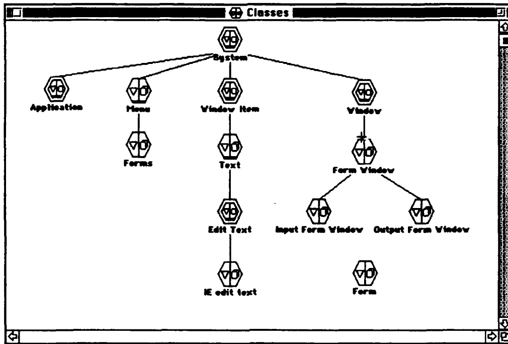
Figure 10: The Form Use Application Program Class Hierarchy
