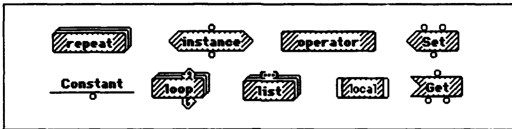
Figure 1. Examples of Prograph Icons
