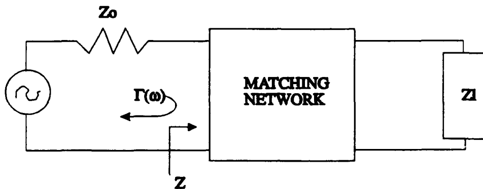
Figure 2.6 Matching Network for an Arbitrary Load Impedance
