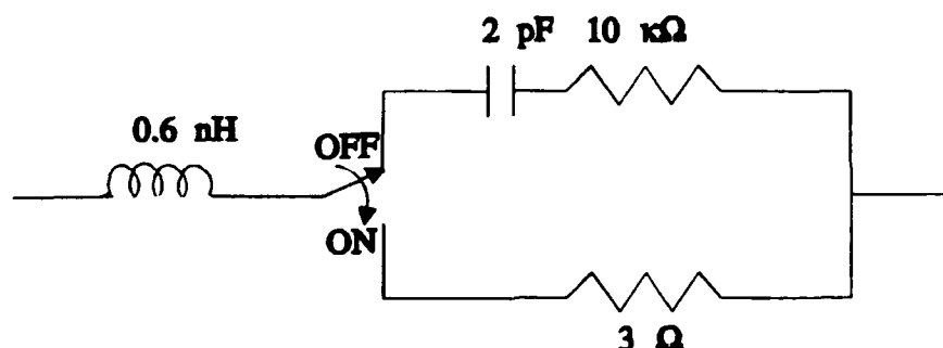
Figure 2.1 PIN Diode Equivalent Circuit
