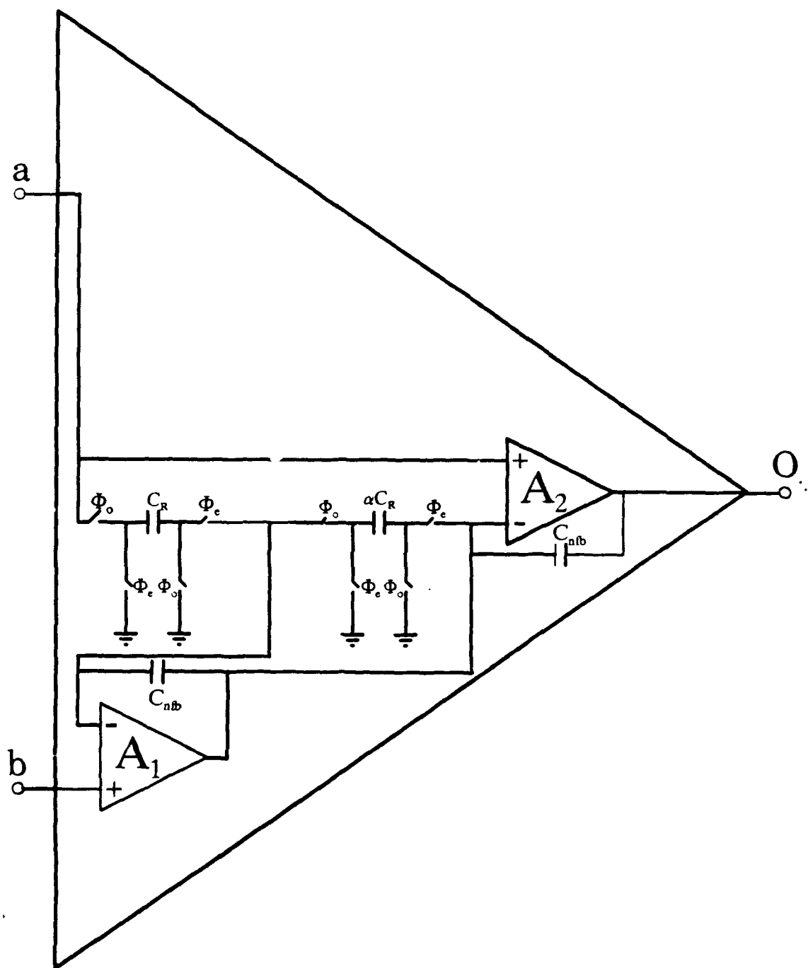
Figure 6.1j Stray Insensitive TSC C20A-1
