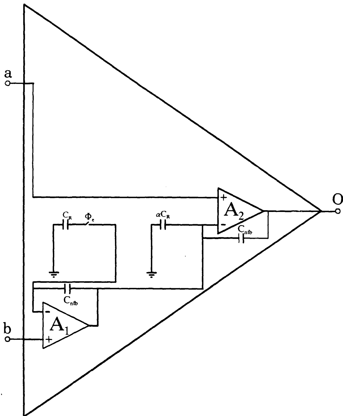
Figure 6.1i TSC C20A-1 with \Phi_c Active and Effective Stray Capacitances
