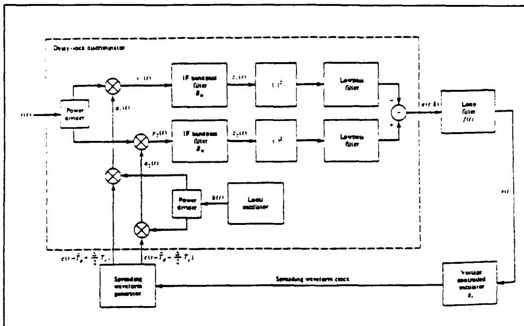
Figure 16. Full-time early-late noncoherent code tracking loop [Ref. 6:p. 434]
