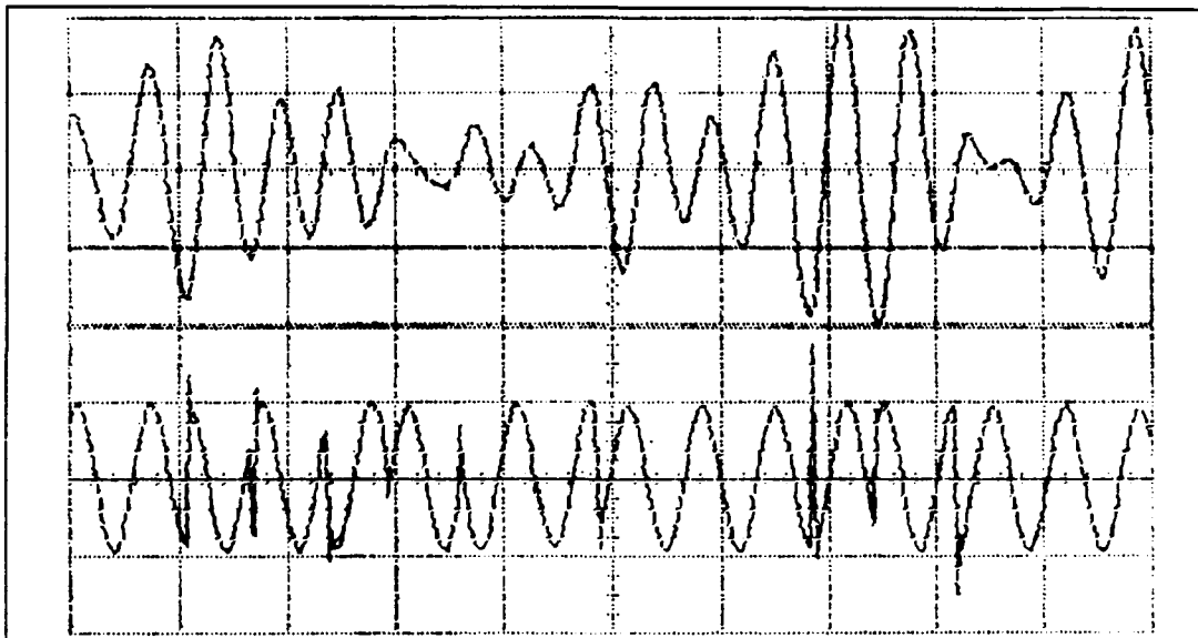
Figure 29. Bottom: Uncorrelated input to BPF, 20 \mu s, 1V; Top: Uncorrelated output from BPF, 20 \mu s, 1V
