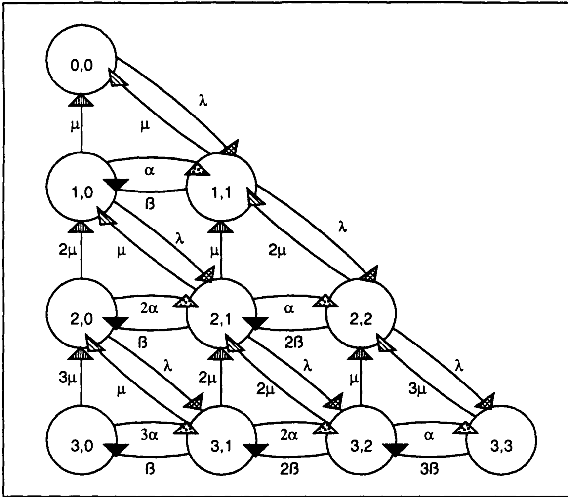
Figure 1. Graphical Representation of Three-Channel Bivariate Erlang System
