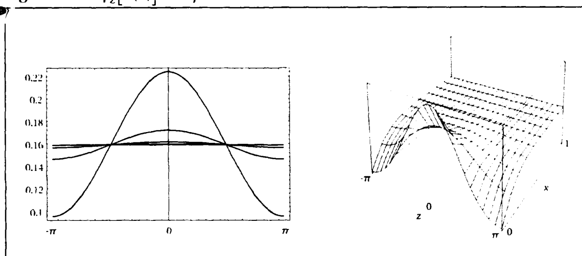
Figure 4.10 f_z[z(x)] for \gamma = 16 .
