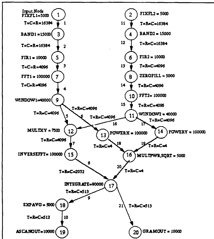
Figure 3.6. Correlator graph
