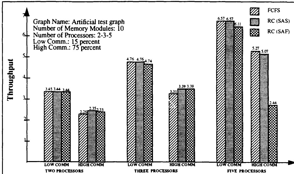
Figure 4.11 The throughput obtain from the artificial test graph.
