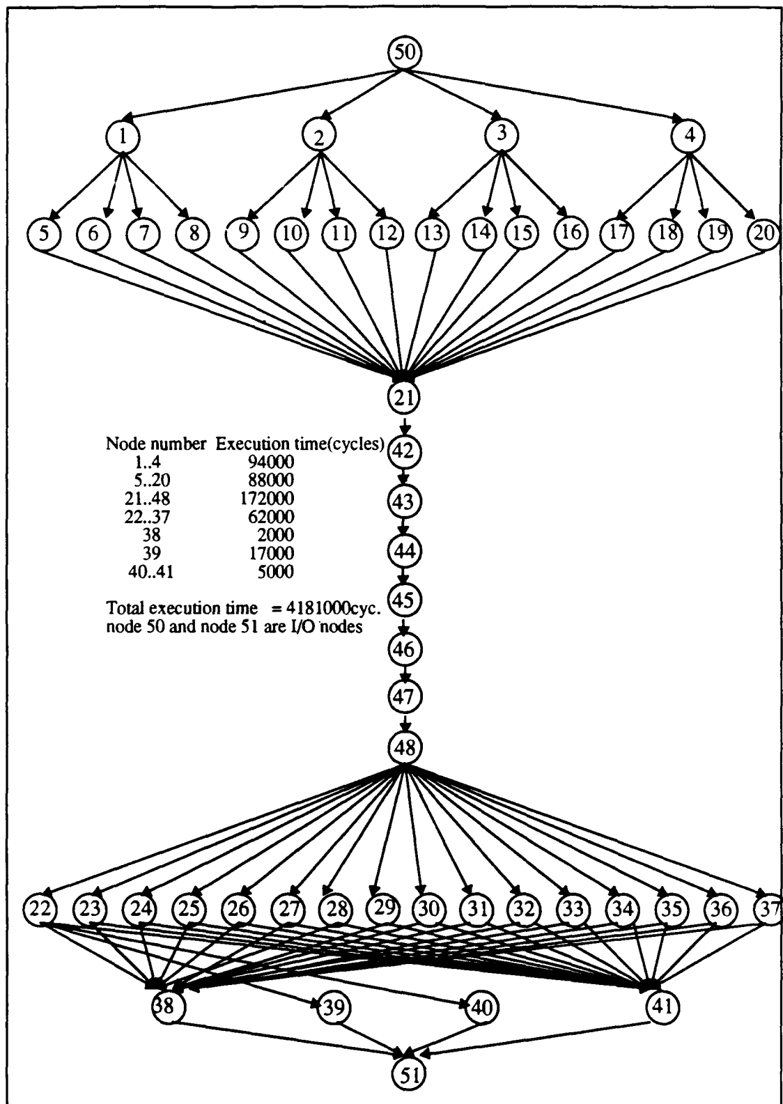
Figure 4.8. Active sonobuoy benchmark graph.
