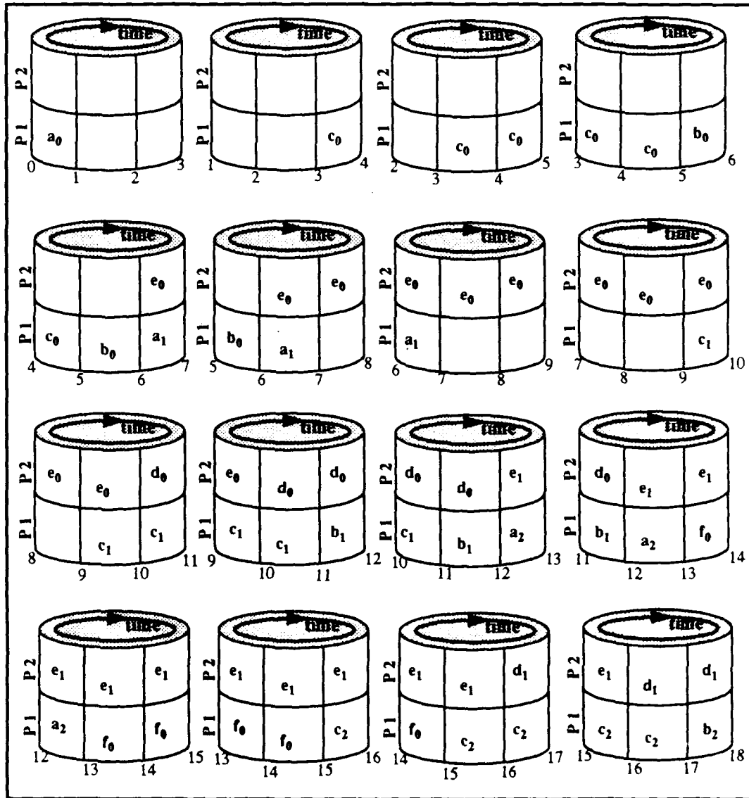
Figure 2.4. Execution of DAG I with Schedule I
