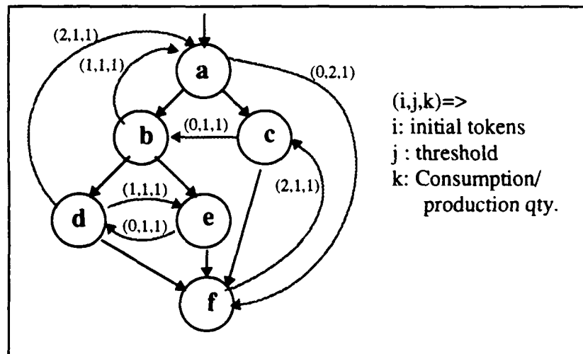
Figure 2.6. A Possible Restructure of DAG I
