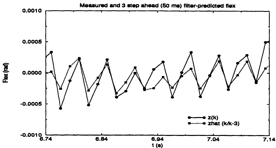
Fig. 6-10: Real barrel flex measurements and 3-step ahead Kalman filter prediction. This shows fairly good muzzle angle prediction when the 20 Hz mode is the dominant.
