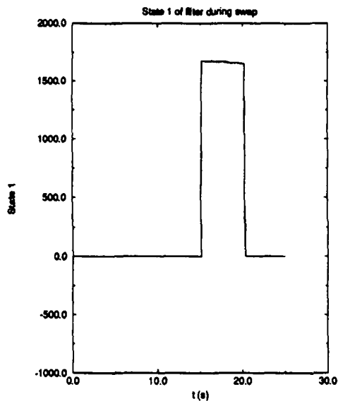
Fig. 5-2: First element of state vector as range becomes valid during t=15 to t=20 .
