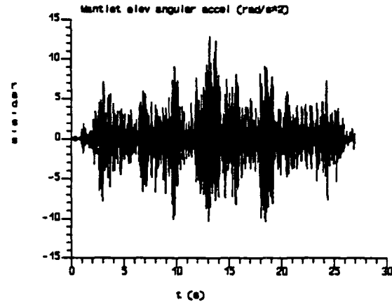
Fig. B-2: Mantlet angular acceleration
