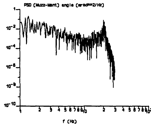
Fig. 6-8: PSD of flex
