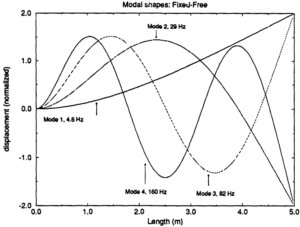
Fig. 6-3: Modal Shape Functions of Fixed-Free Hollow Tube
