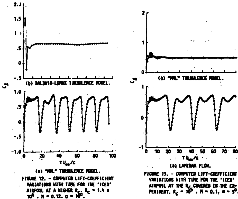
Figure 13. Computed Lift Coefficient Variations with Time
