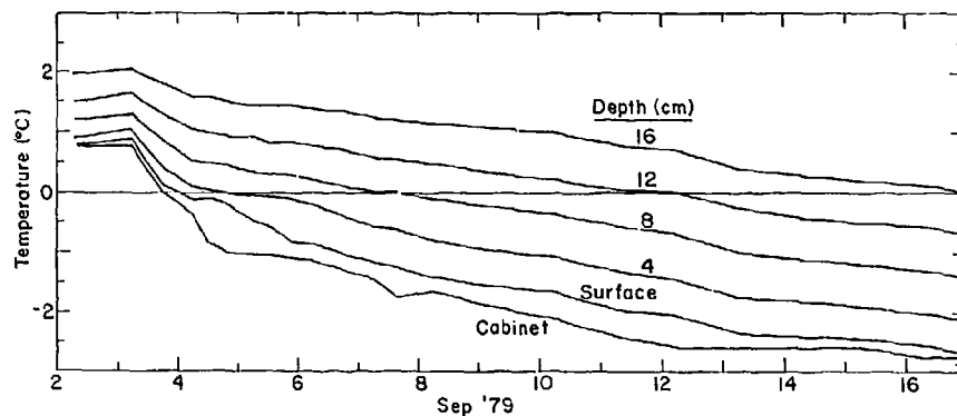
d. Temperatures during the test.
