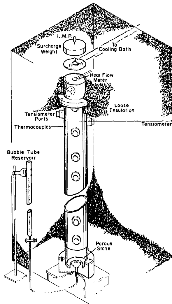
Figure 5. CRREL soil column.
