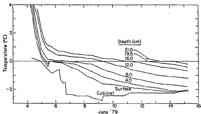
d. Temperatures during the test.
