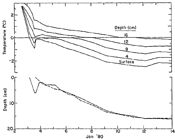
d. Temperatures and frost penetration during the test.
