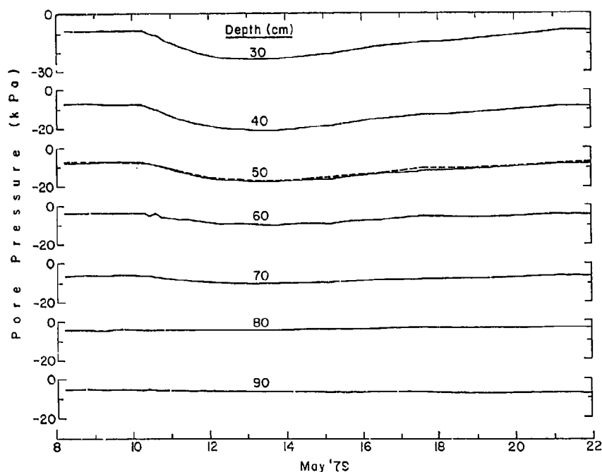
c. Pore water pressures, 30- to 90-cm depths.
