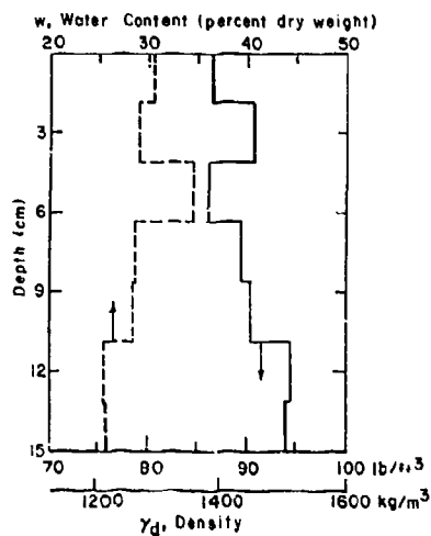
e. Moisture contents and densities after the test.
