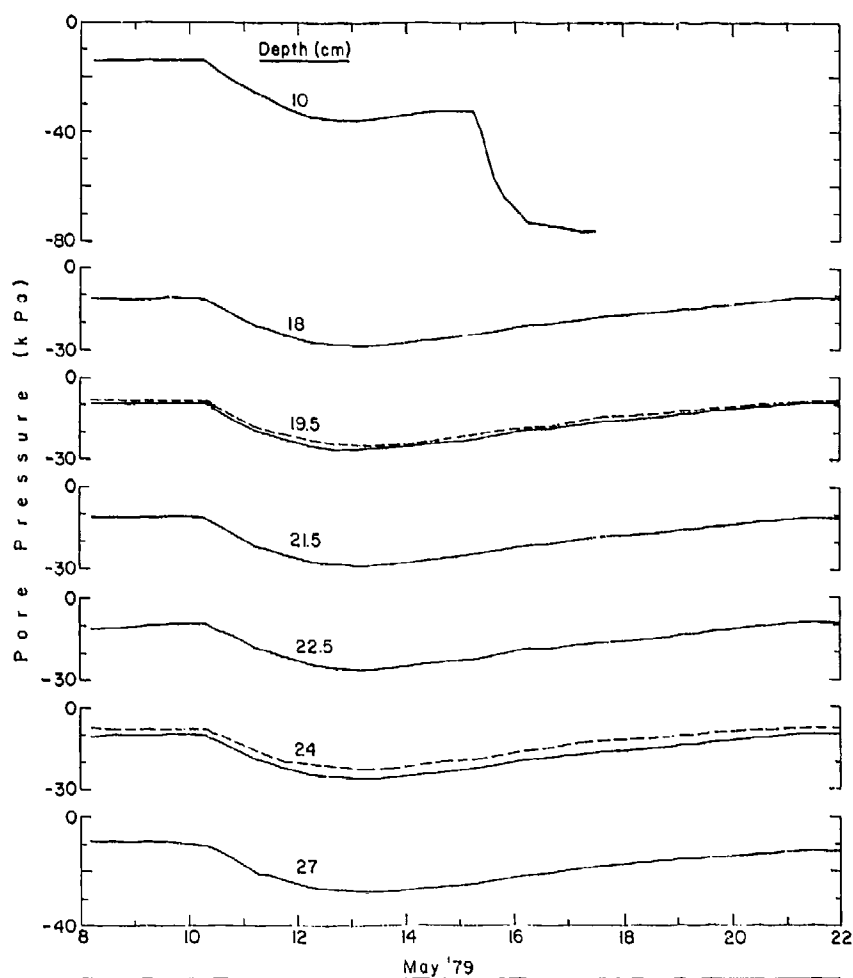
b. Pore water pressures, 10- to 27-cm depths.
