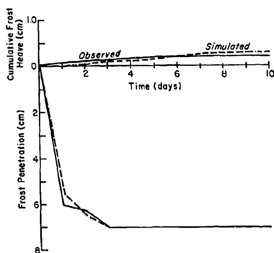
b. Surcharge of 34.5 kPa.
