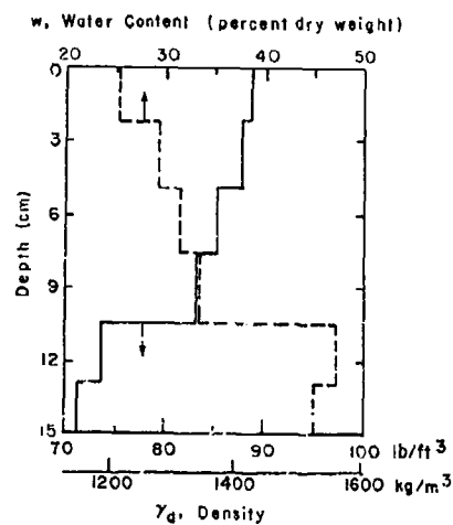
e. Moisture contents and densities after the test.
