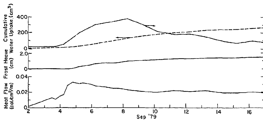
a. Surface heat flux, total frost heave and water uptake.
