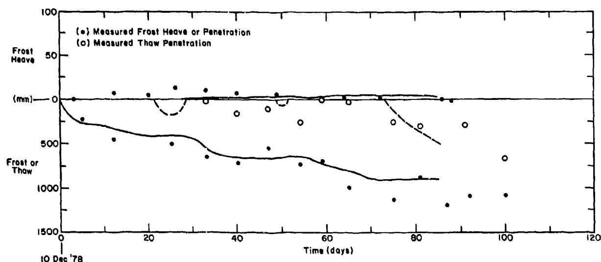
Figure 13 (cont'd). Simulated frost heave, thaw settlement, frost penetration and thaw penetration, 1978-79.
