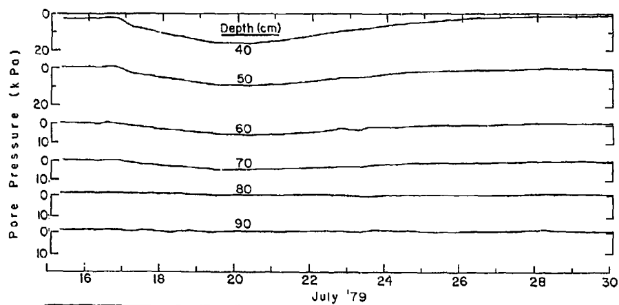
c. Pore water pressures, 40- to 90-cm depths.
