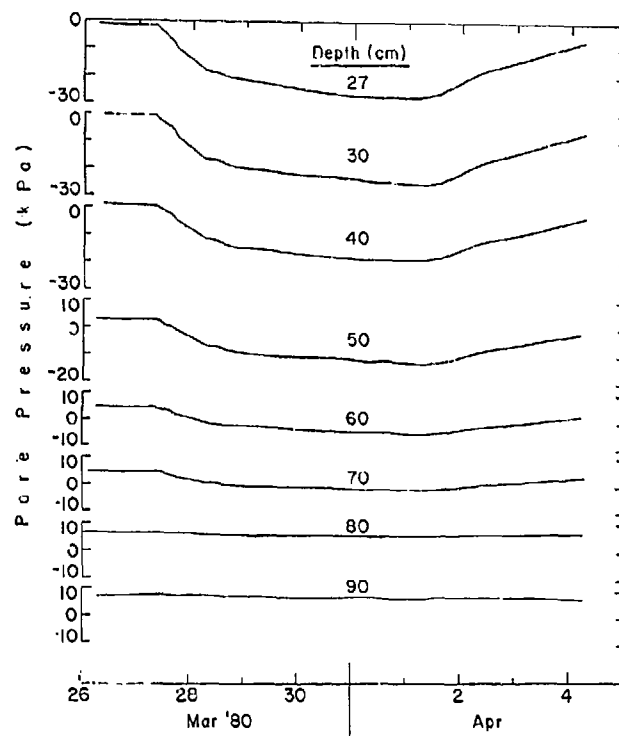
c. Pore water pressures, 27- to 90-cm depths.
