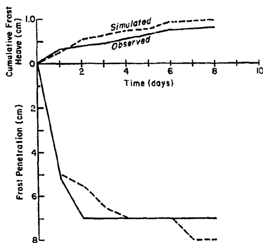
a. Surcharge of 3.45 kPa.
