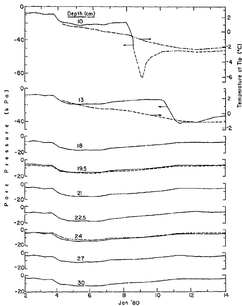
b. Pore water pressures, 10- to 30-cm depths.
