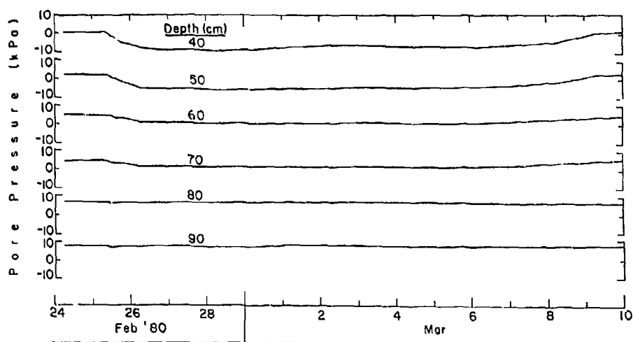
c. Pore water pressures, 40- to 90-cm depths.
