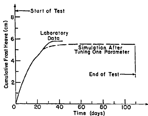
a. Surcharge of 3.45 kPa.
