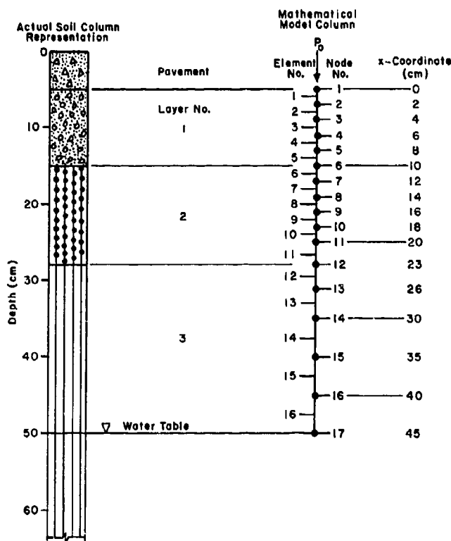
Figure 21. Example soil profile divided into finite elements.
