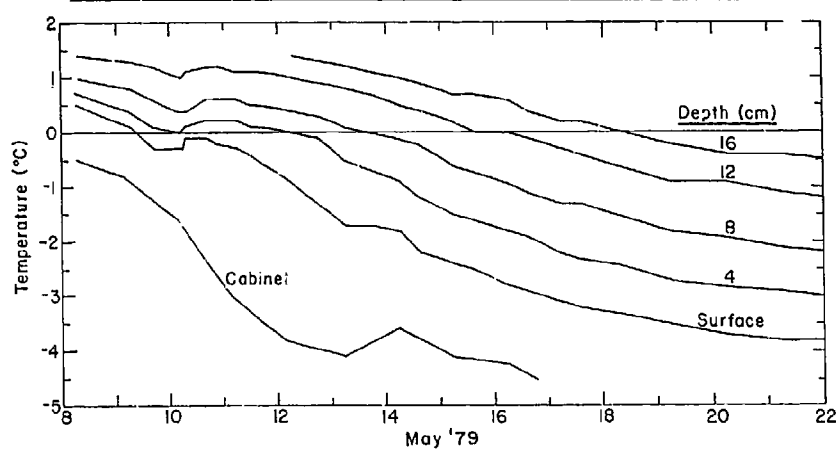
d. Temperatures during the test.
