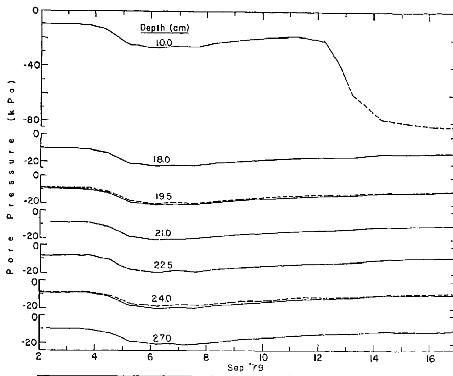
b. Pore water pressures, 10- to 27-cm depths.
