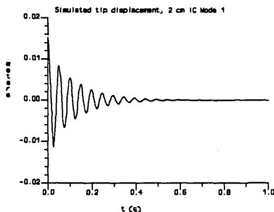
Fig. 6-4: Simulated tip motion
