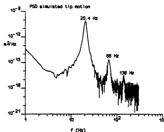
Fig. 6-5: PSD of simulated tip motion
