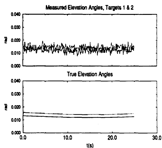
Fig. 5-9 Measured and true elevation angles, two targets
