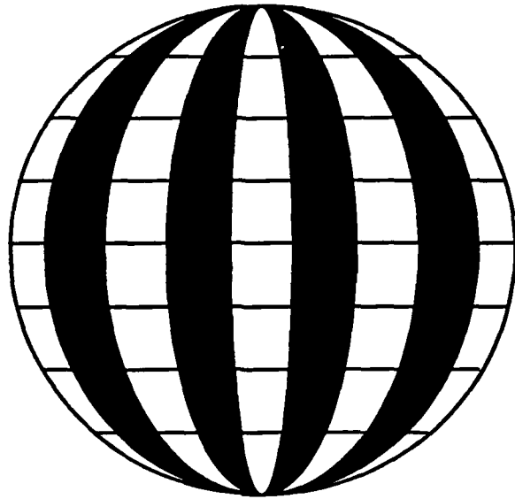
Figure 2.5 Sectorial Harmonics
