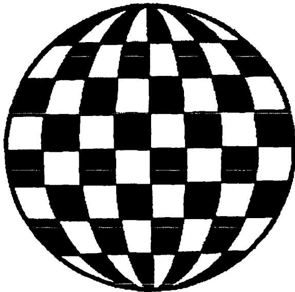
Figure 2.6 Tesseral Harmonics
