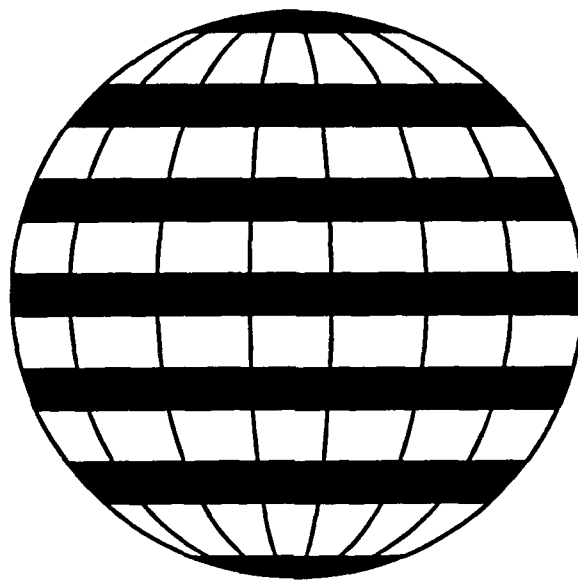
Figure 2.2 Zonal Harmonics
