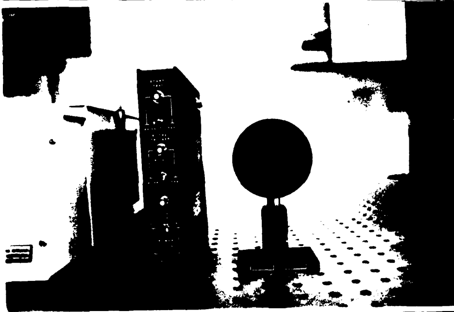
SPIRICON, INC. LASER PROBE LINEAR DETECTOR ARRAY (PYROELECTRIC) WITH CONTROLLER MODEL NO. LP-256-11 (256 ELEMENTS IN 25.6 MM LONG ARRAY)
