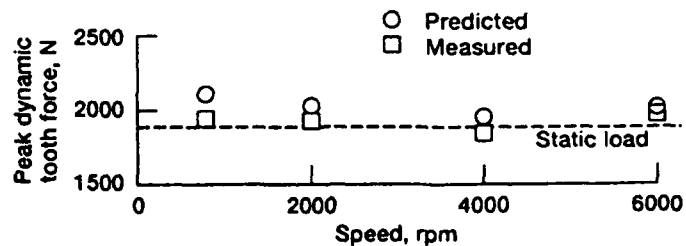
Figure 13.—Comparison between predicted and measured peak dynamic tooth load at 110-percent torque and four speeds.
